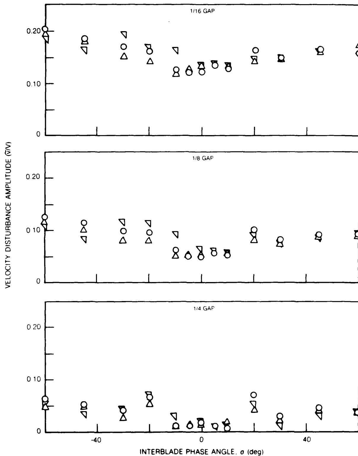
Fig. 6 First Harmonic Amplitude of Inlet Plane Disturbance as a Function of Interblade Phase Angle ( \alpha_M = 6 deg). k_c : \nabla , 0.07; \circ , 0.13; \triangle , 0.19
