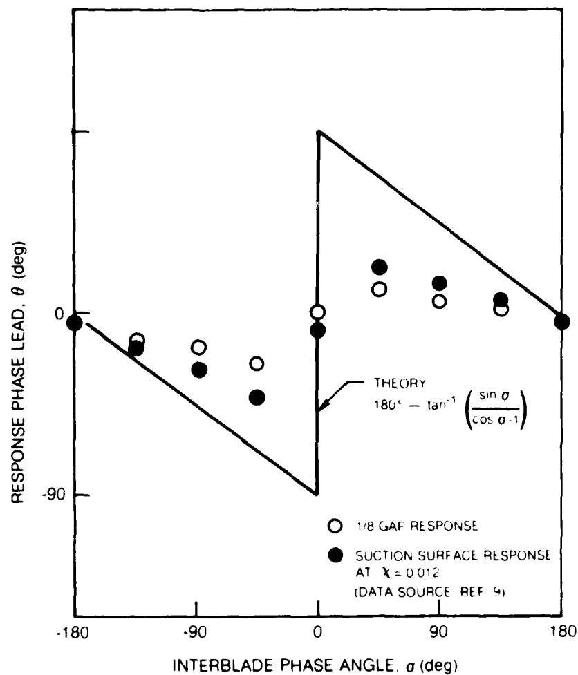
Fig. 17 Comparison of Trend in Inlet Area Phase Lead with First Harmonic Components of Inlet Plane Disturbance (1/8 Gap Station) and Suction Surface Response ( \chi=0.012 ). k_c = 0.12 ; \alpha_M = 2 deg; \bar{\alpha} = 2 deg; \tau/c = 0.75
