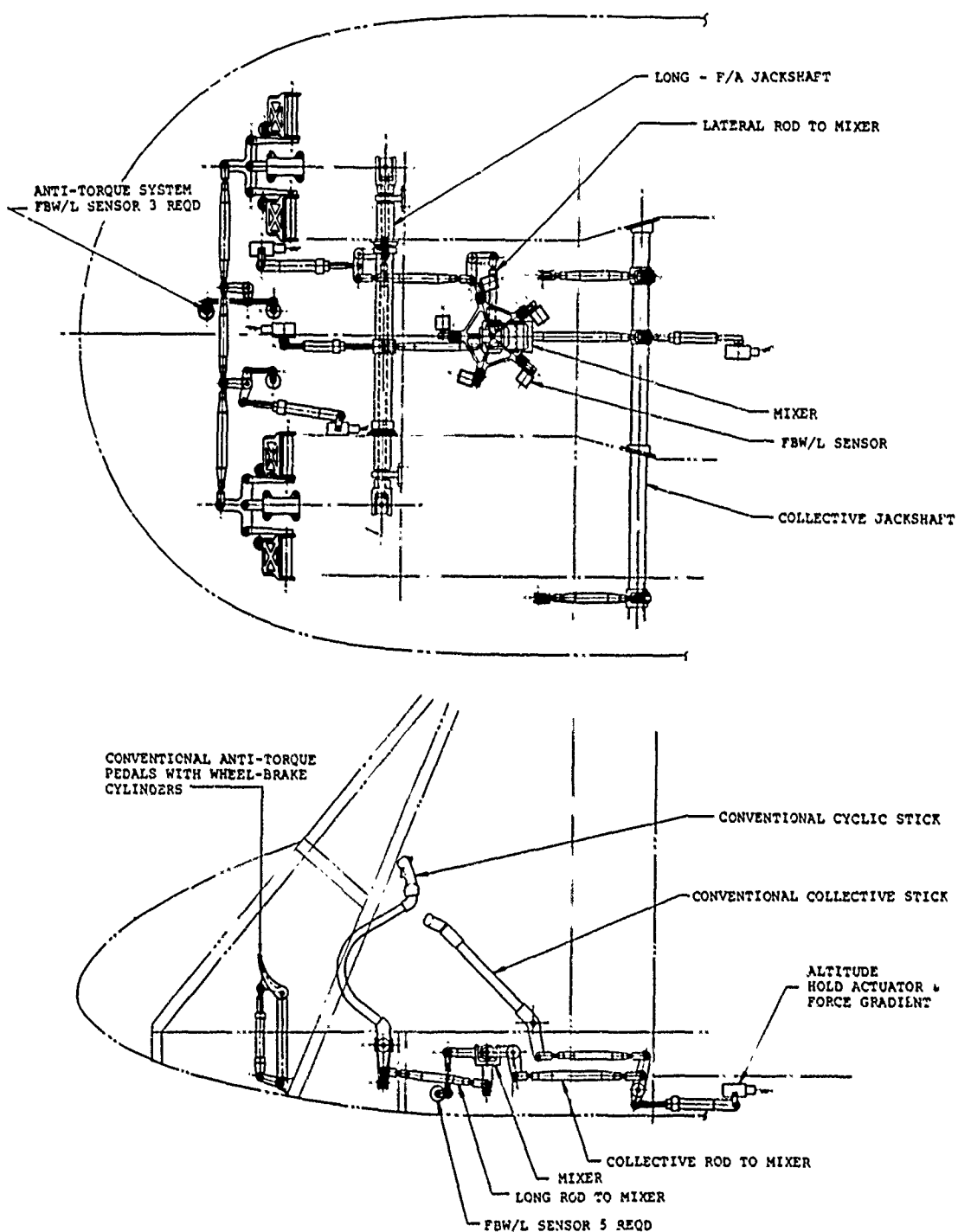
Figure 13. Mechanical layout for FBW/L control system.
