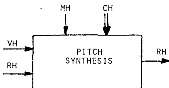
Figure 22. Pitch synthesis
