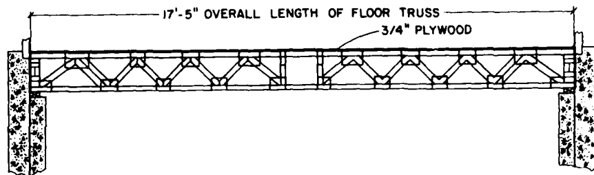
Figure 4.—Floor-truss design subjected to test conditions of ASTM E-119. Upper chord was loaded with tanks simulating a uniform load of 55.1 lb/ft 2 that resulted in a combined live and dead load of 60 lb/ft 2 .
