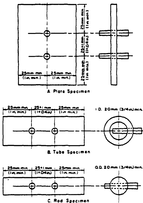
FIGURE 7.3: TAPER-PIN ELECTRODES
