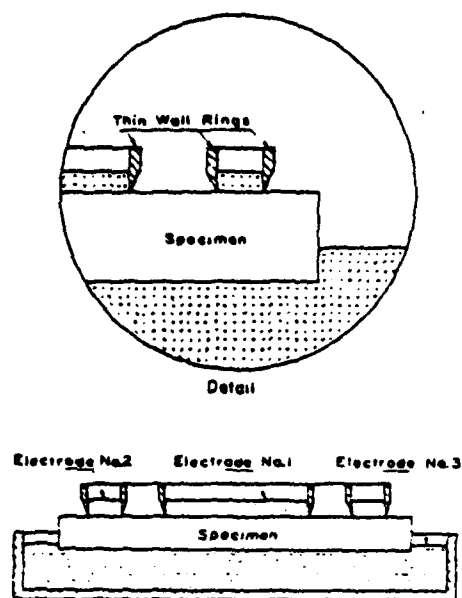
FIGURE 7.5: MERCURY ELECTRODES FOR FLAT, SOLID SPECIMENS
