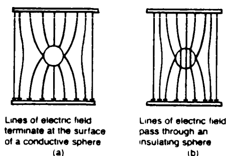
FIGURE 2.4: (A) CONDUCTOR AND (B) INSULATOR IN A UNIFORM ELECTRIC FIELD
