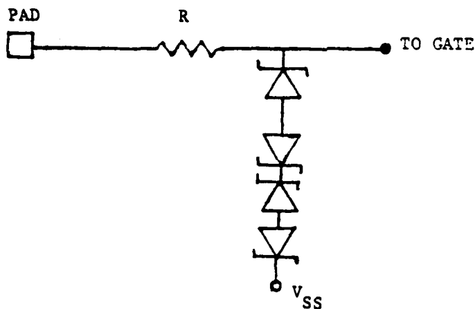
FIGURE 10.14: ZENER DIODES
