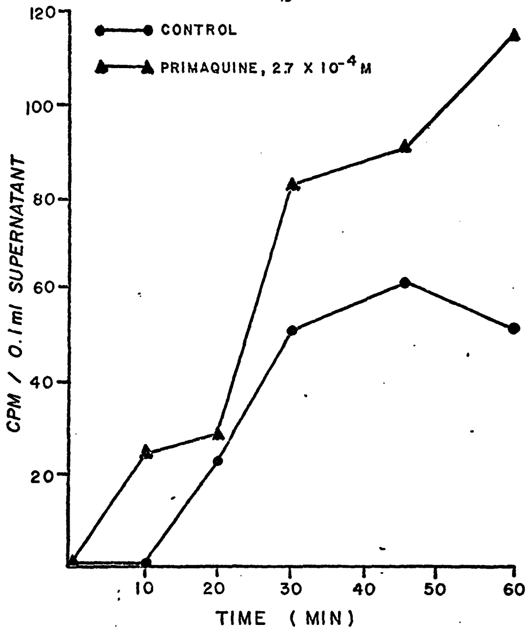
Figure 20. Release of ^{14}\text{C} -amino acids from intracellular pools in the presence and absence of primaquine.
