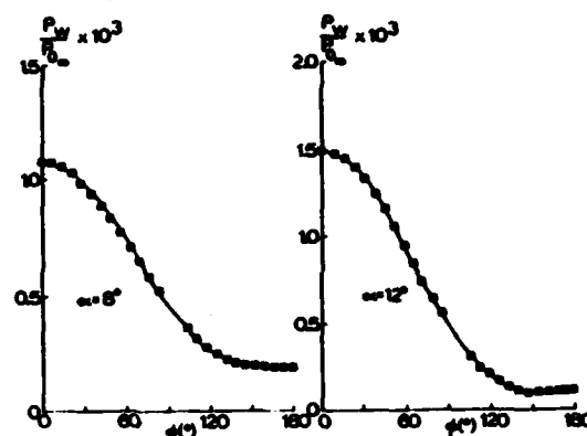
Fig. 6a. Surface Pressure at Moderate Incidence.
