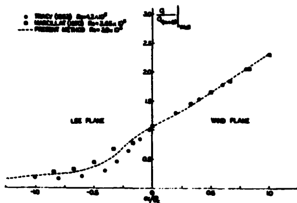
Fig. 5a. Symmetry Plane Heat Transfer - Moderate Incidence.
