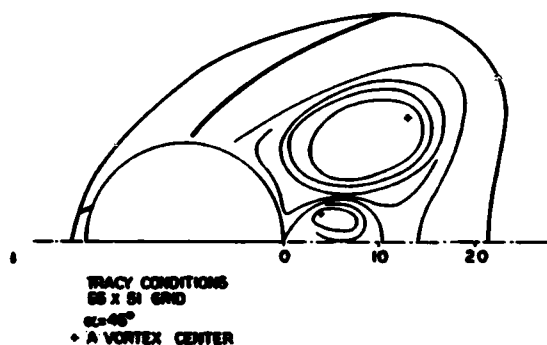
Fig. 13b. Flow Pattern for \alpha = 45^\circ .
