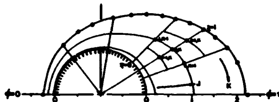
Fig. 2. Difference Grid in the Cross Plane.
