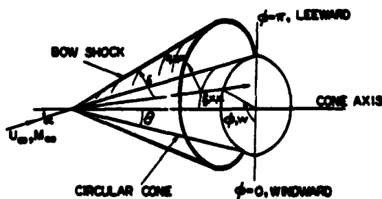
Fig. 1. Flow Geometry.
