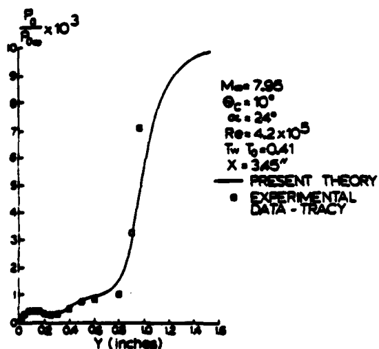
Fig. 7c. Stagnation Pressure at the Lee Plane - \alpha = 24^\circ .
