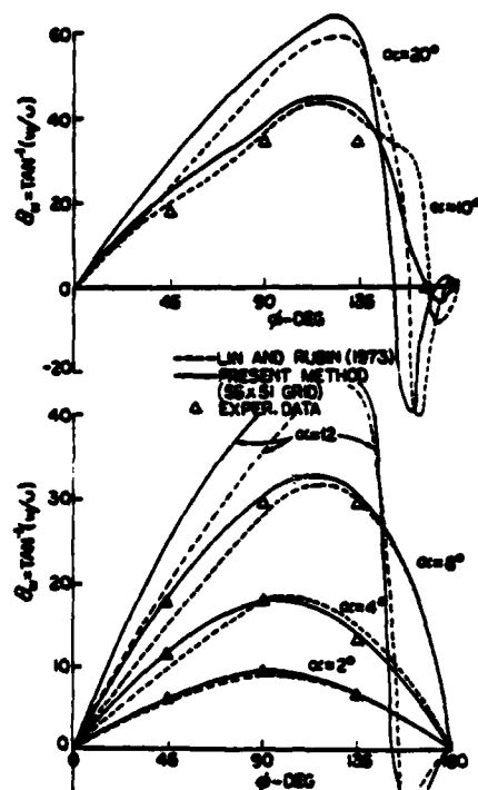
Fig. 8a. Surface Streamline Inclination - Moderate Incidence.
