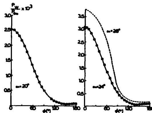
Fig. 6b. Surface Pressure at Large Incidence.
