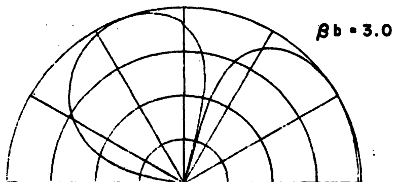
Figure 5-2. Vertical pattern at \phi = 0^\circ .
