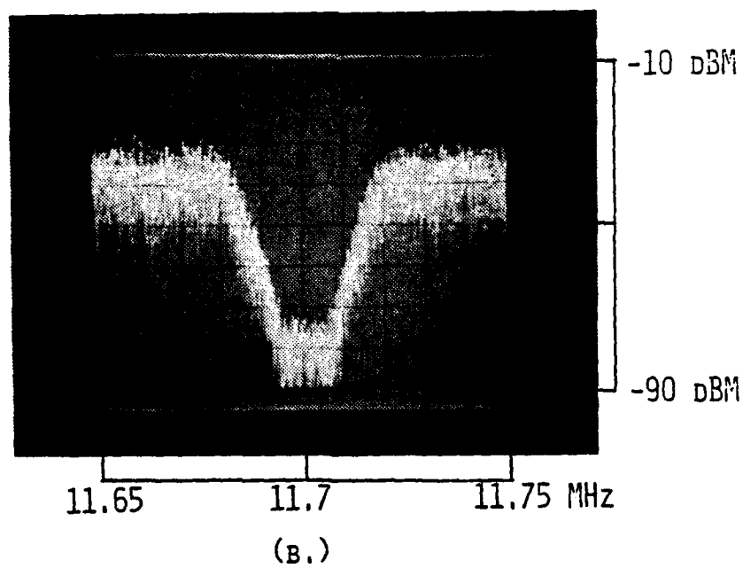
Figure 7. 11.7 MHz Stopband, Multicoupler (A.) Input (B.) Output, NPR = 48.2 dB
