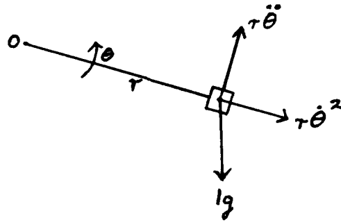
Fig C1 Accelerations acting on a transducer rotating in the earth's gravitational field about O in a vertical plane
