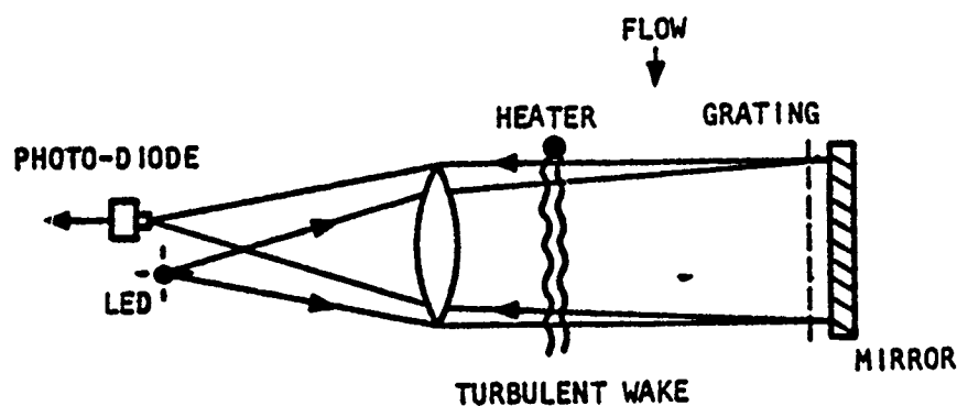
Fig. 6 The Optical Convolution Velocimeter [2]
