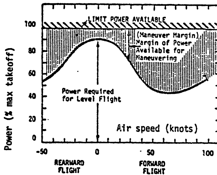
Fig. 3 Power requirement in level flight
