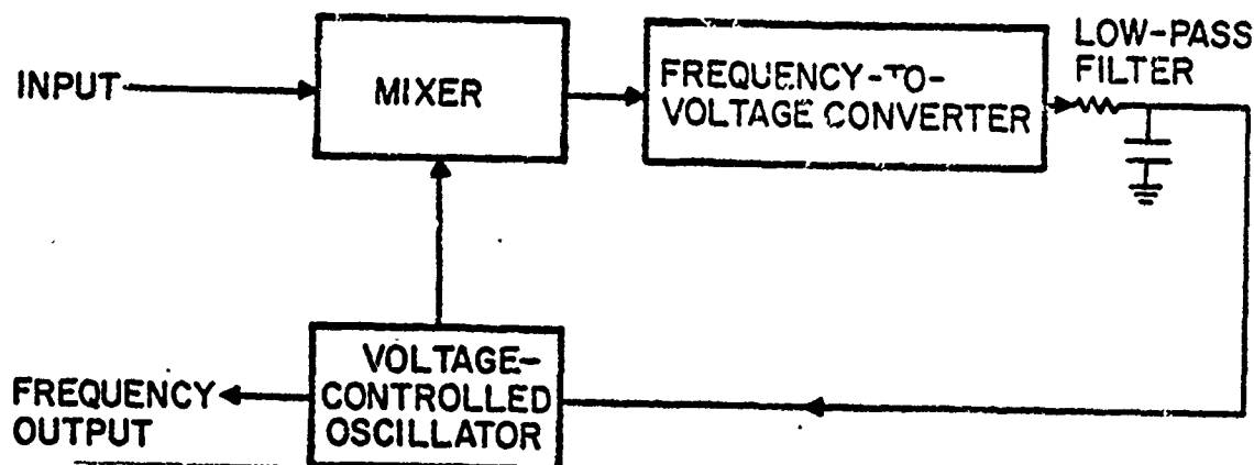
Fig. 10 Frequency-Locked Loop [2]
