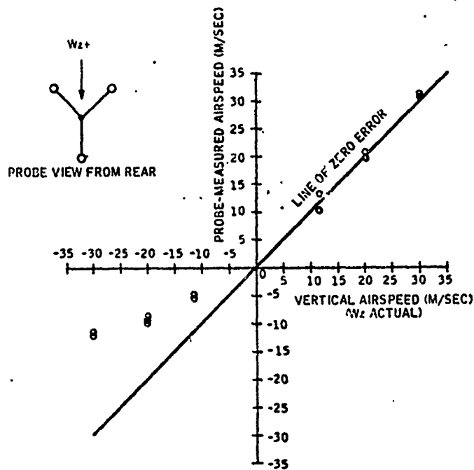
Figure 21c Wind Tunnel Performance (Vertical Direction)
