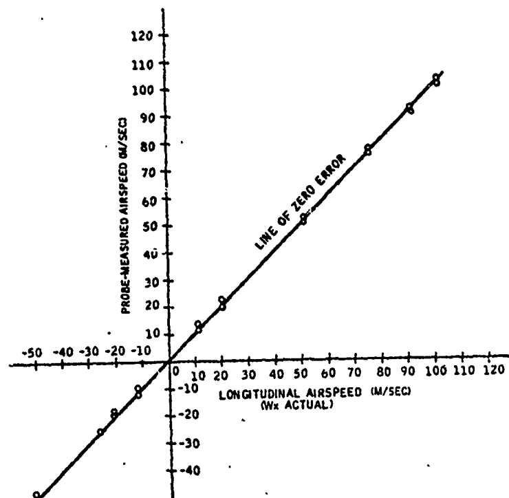
Fig. 21a Wind Tunnel Performance (Longitudinal Direction) [5]
