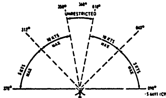
Fig. 2 Wind limitation profile for launch and recovery, H-3 helicopter.
