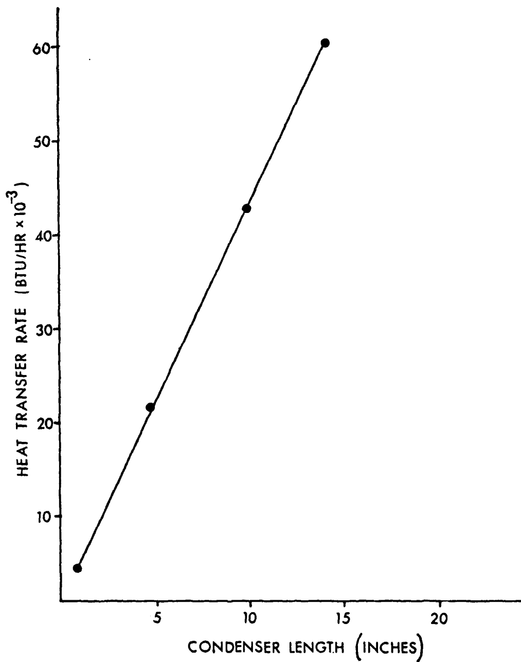
Figure 10. Heat Transfer Rate (Q) vs. Condenser Length
