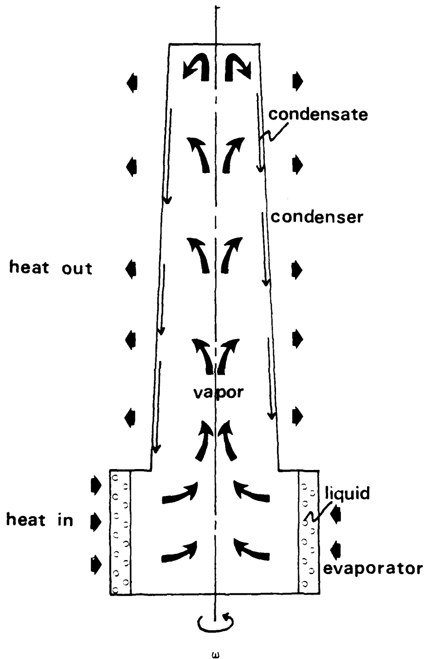
Figure 1. Schematic Drawing of a Rotating Heat Pipe
