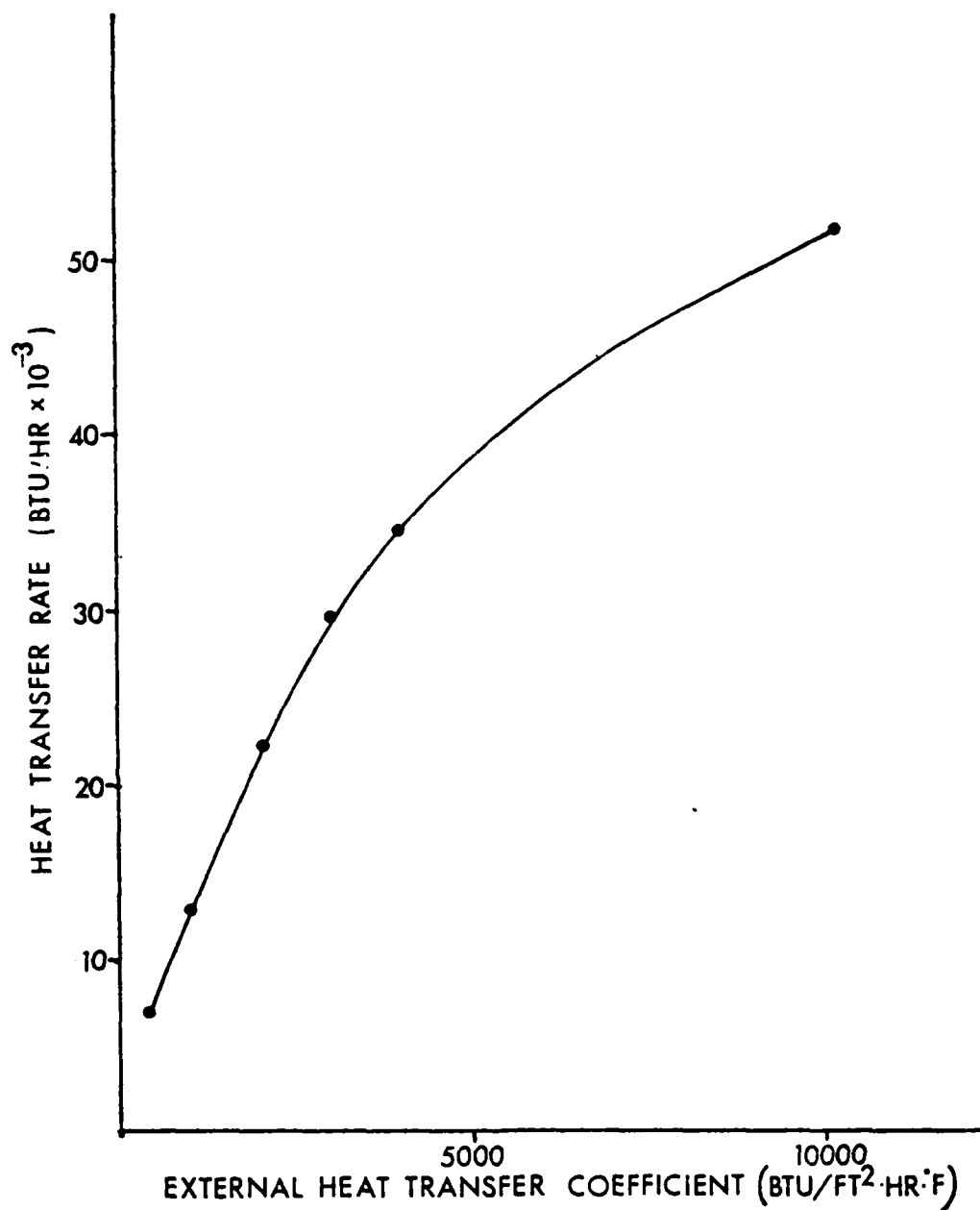
Figure 9. Heat Transfer Rate (Q) vs. External Heat Transfer Coefficient
