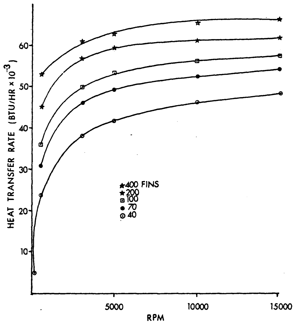
Figure 8. Heat Transfer Rate (Q) vs. RPM
