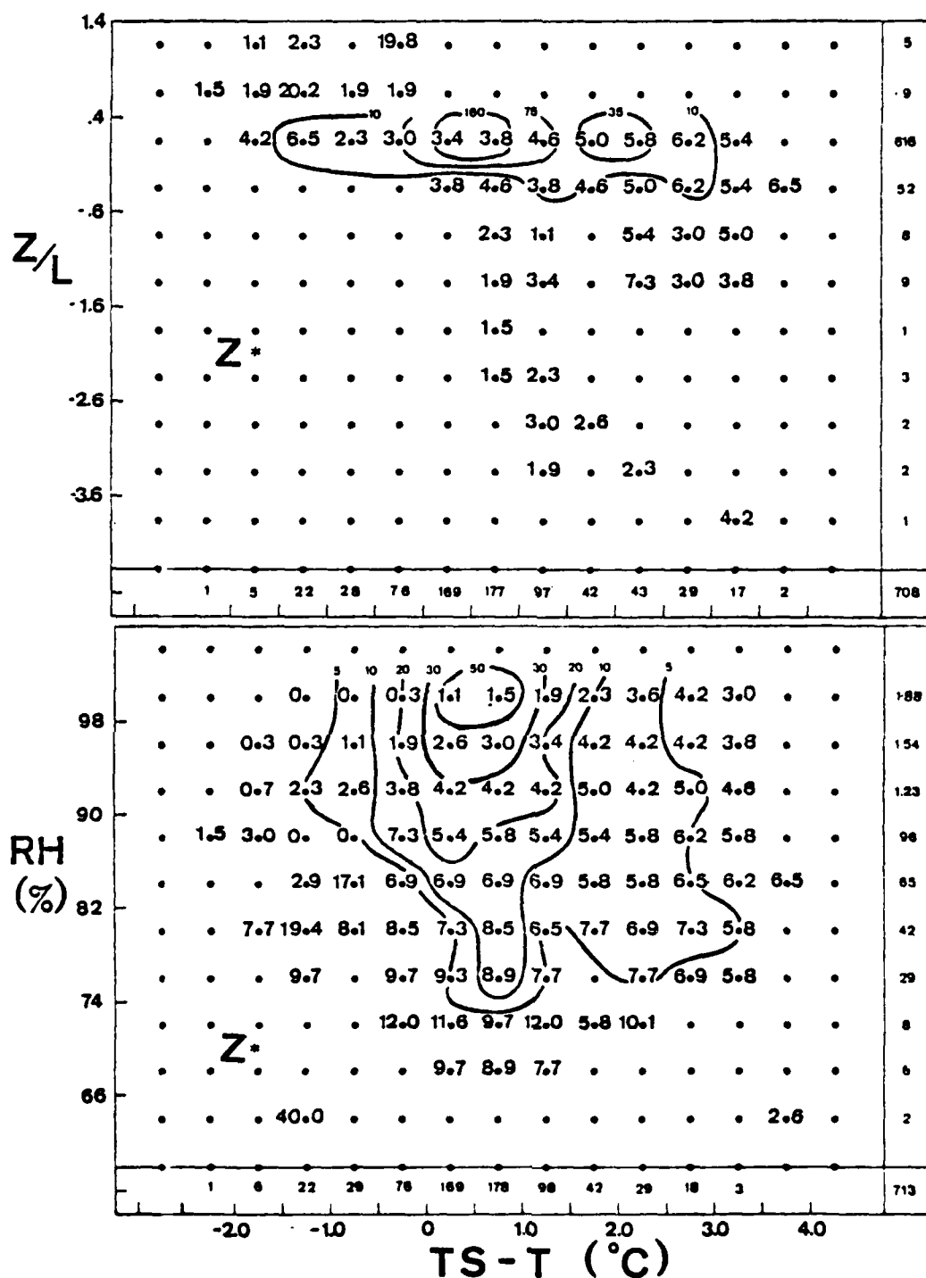
Figure 8 (top). JDF of Z/L and Figure 9 (bottom) JDF of RH and Ts-T to CMF of Z^* .
