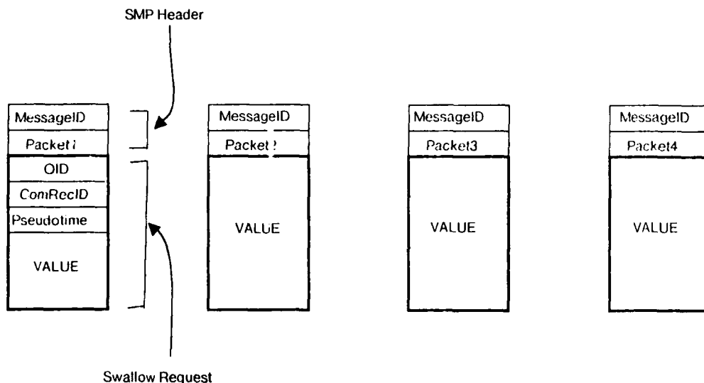
Figure 3-3: Structure of a Create-Token Message
