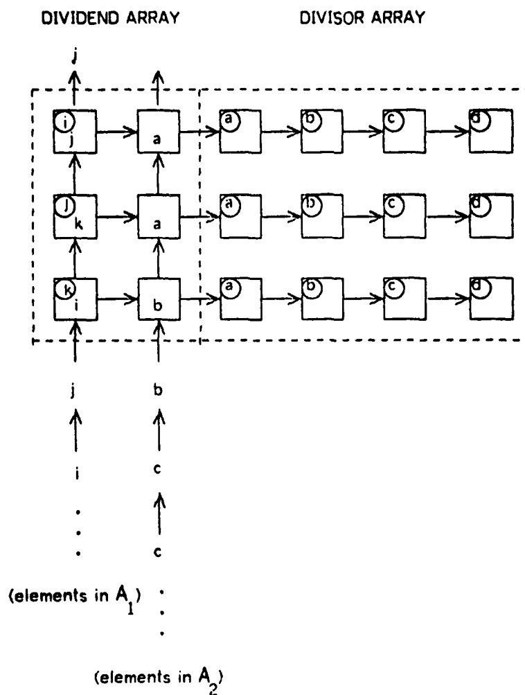
Figure 7-2: Division array (in operation).
