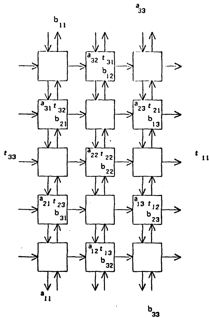
Figure 3-4: Data moving through the comparison array.
