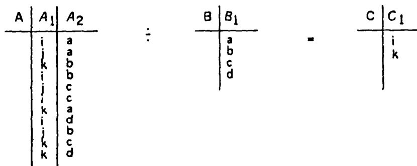
Figure 7-1: Example of relational division
