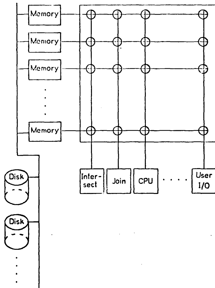
Figure 9-1: Systolic database system using crossbar switch.
