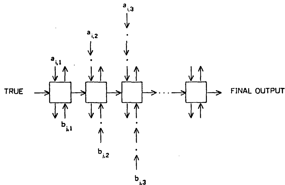
Figure 3-1: Tuple comparison array.
