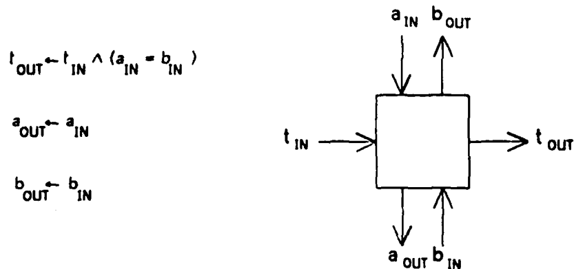
Figure 3-2: Individual comparison processor.
