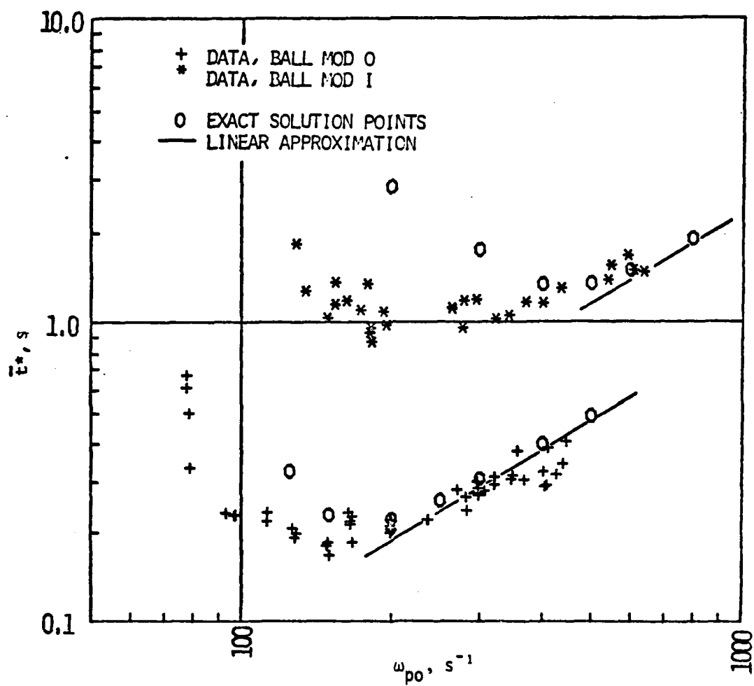
Figure 22. Presentation of experimental results showing comparisons with exact and approximate solutions. Gravity load only.
