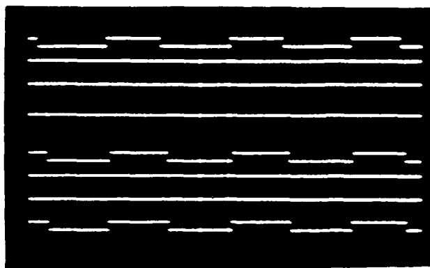
Figure 3.24 Eight Control Signals to Demonstrate The Function of Distributed Controller For Arbitration of Intra-Star and Intra-Cluster Communication
