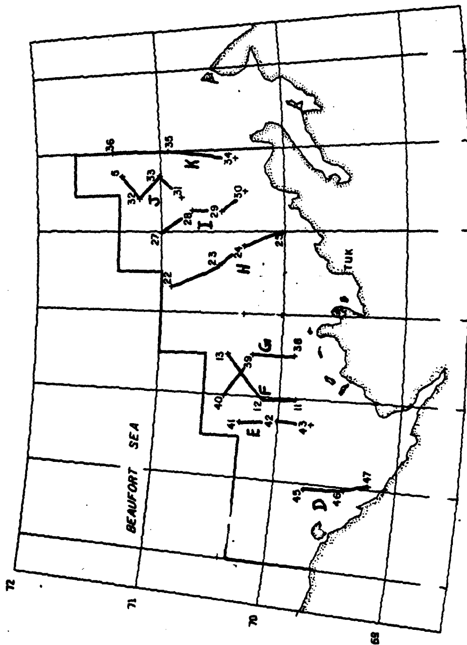
Figure 77: Location of oceanographic vertical cross-sections D, E, F, G, H, I, J, K in the study area during August 1975.
