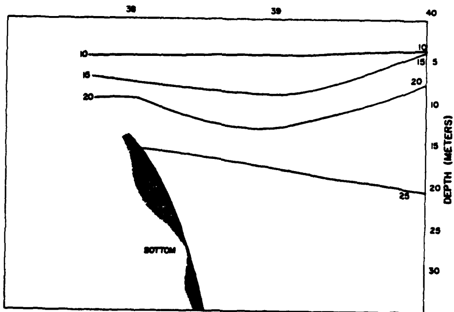
DENSITY CROSS-SECTION 1975
