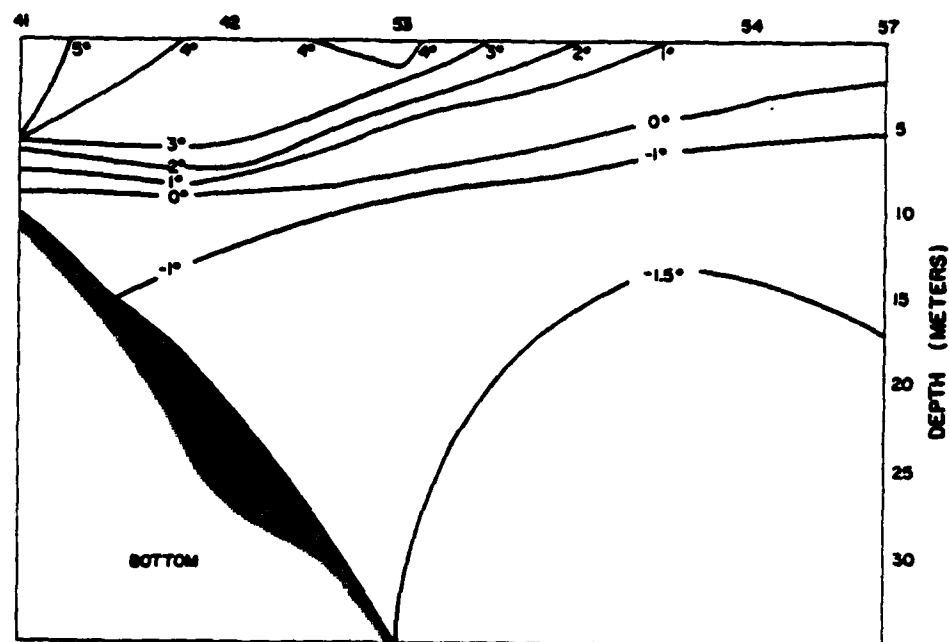
TEMPERATURE CROSS-SECTION 1974
