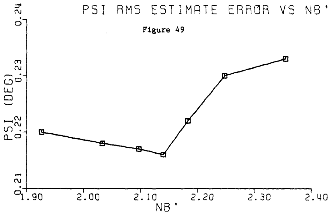
Figures 49 & 50. Sensitivity of \bar{\Psi} and \bar{V}_{\beta_g} rms estimate errors vs variation in N'_g stability derivative.
