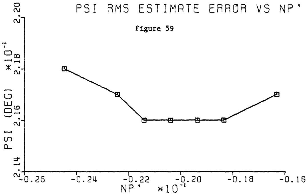
Figures 59 & 60. Sensitivity of \bar{\psi} and V_{\beta_0} rms estimate errors vs variation in N'_p stability derivative.
