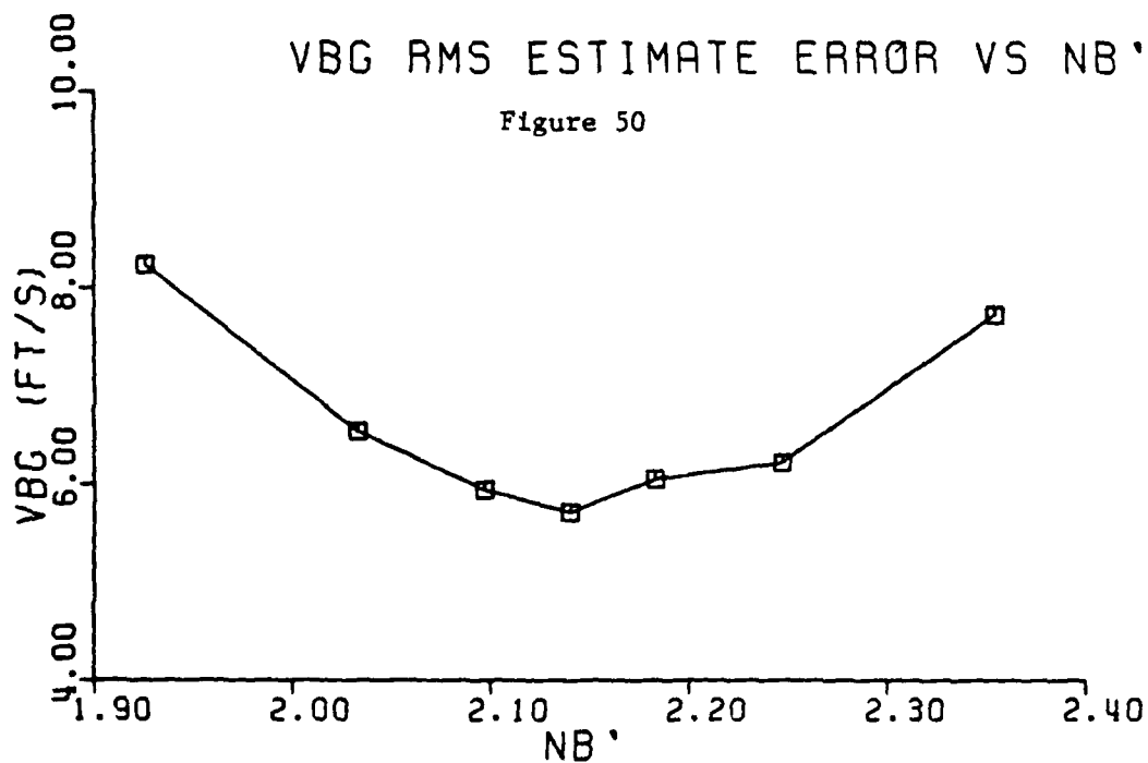
Figures 49 & 50. Sensitivity of \bar{\Psi} and \bar{V}_{\beta_g} rms estimate errors vs variation in N'_g stability derivative.
