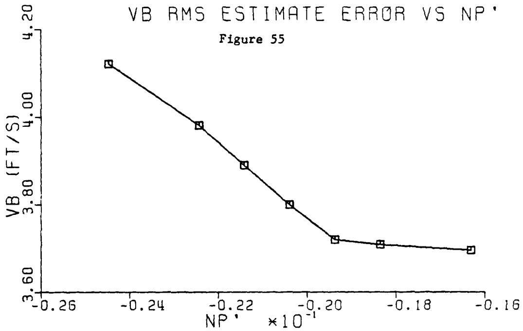
Figures 55 & 56. Sensitivity of \bar{V}_\beta and \bar{r} rms estimate errors vs variation in N'_p stability derivative.
