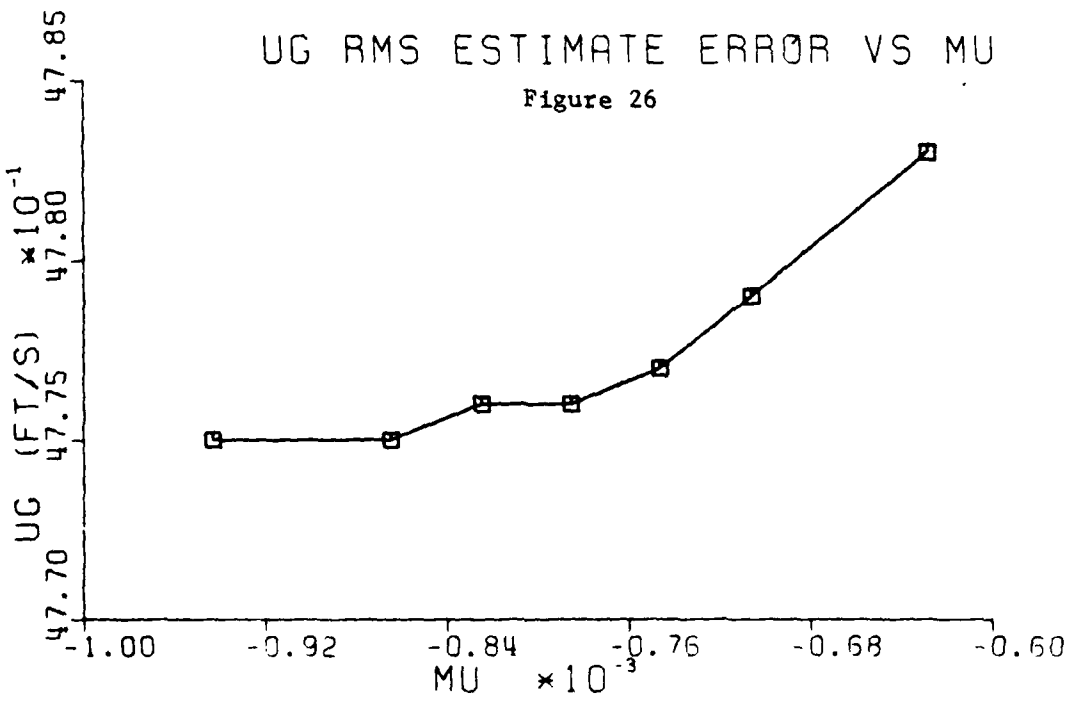
Figures 25 & 26. Sensitivity of \bar{w}_g and \bar{u}_g rms estimate errors vs variation in Mu stability derivative.
