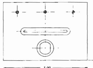
CARD READER FACEPLATE
