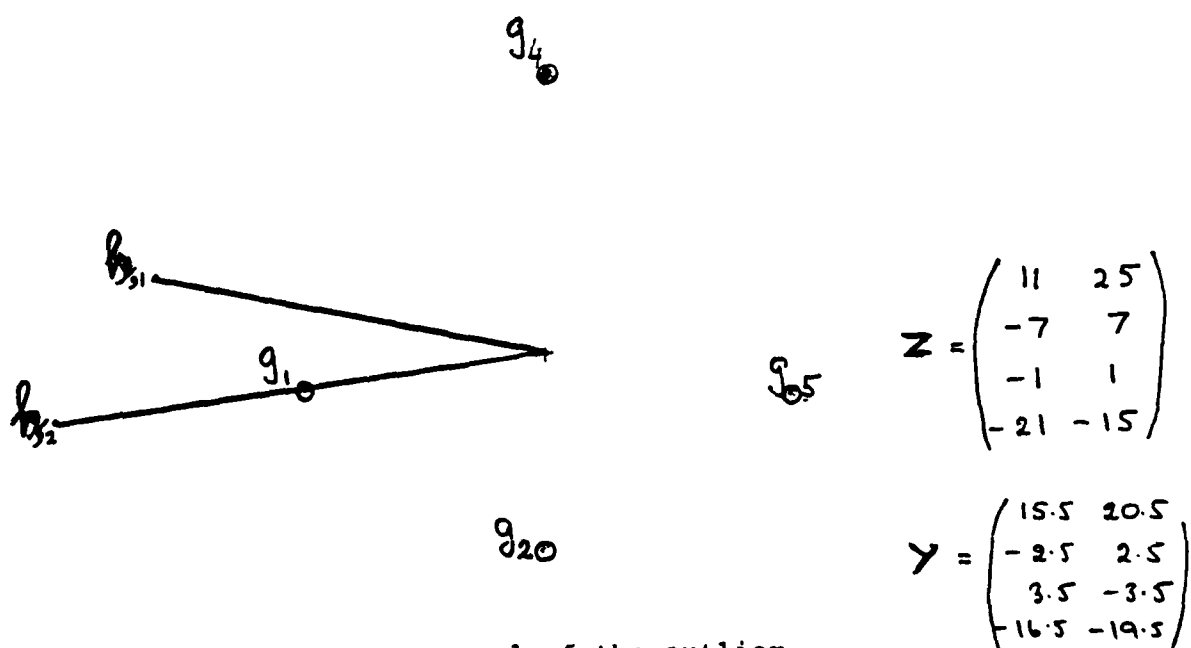
Fig. 11b The biplot after removal of the outlier
