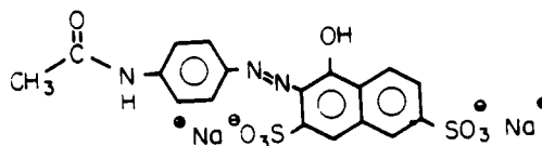
Kiton Red S (Original Azo Dye Structure)
