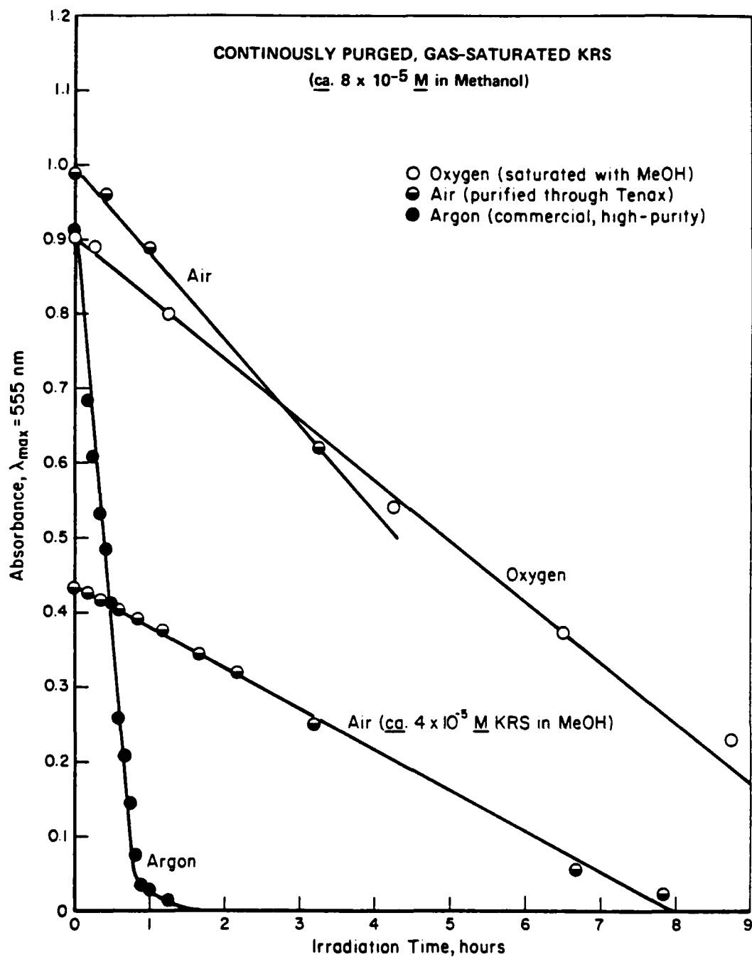
FIGURE 7. RATES OF PHOTBLEACHING OF CONTINUOUSLY PURGED, GAS-SATURATED KRS IN METHANOL
