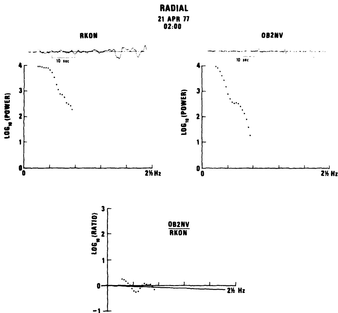
Figure 28. Time traces, power spectra and power spectral ratios for short period S waves observed at SDCS stations RKON and OB2NV, 21 April 1977 event, radial component.
