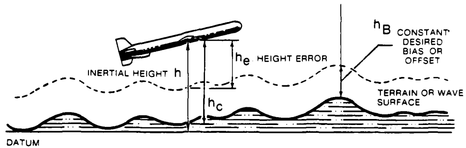
FIGURE A1. CRUISE MISSILE FLYING ABOVE TERRAIN
