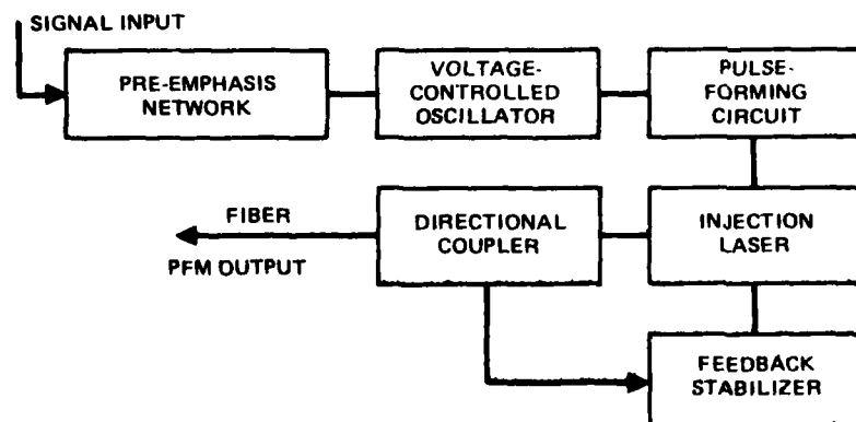
Figure 14. Block diagram of the PFM transmitter used in the NOSC PFM brassboard data link.
