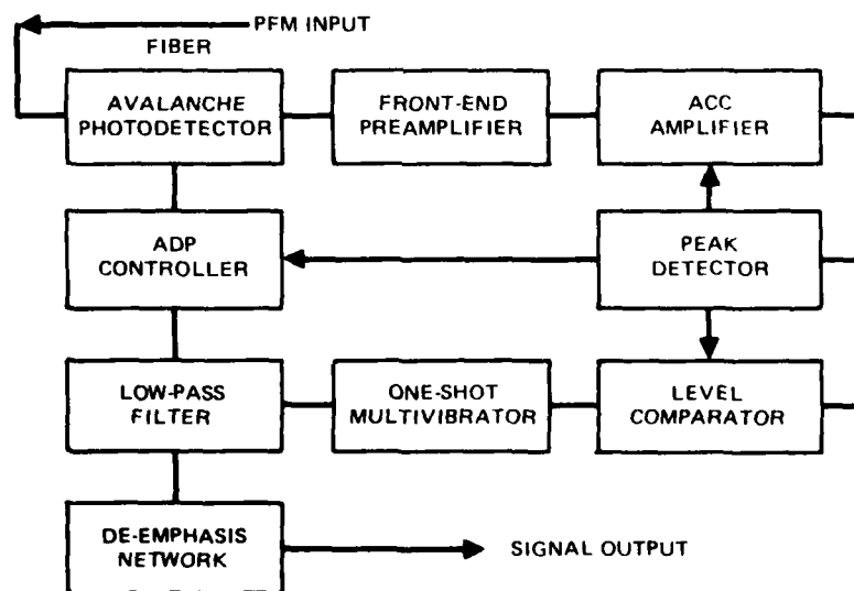
Figure 15. Block diagram of the PFM receiver.
