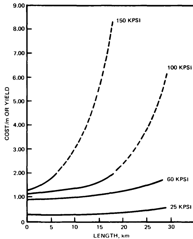
Figure 4. Typical yield curves for fiber-optic links.
