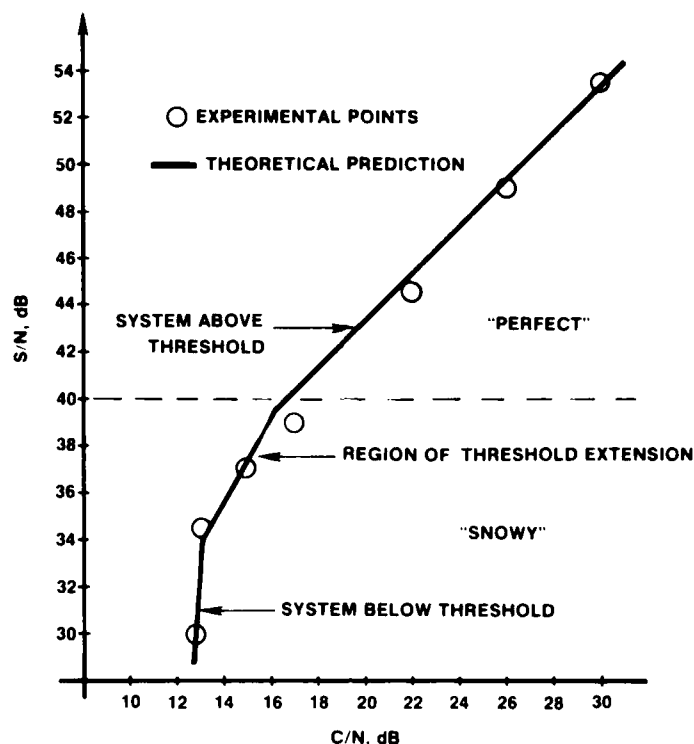
Figure 16. Receiver operating characteristics compared with theoretical predictions.
