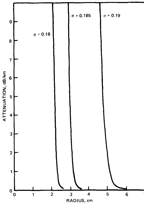
Figure 9. Sensitivity of various modes to curvature.
