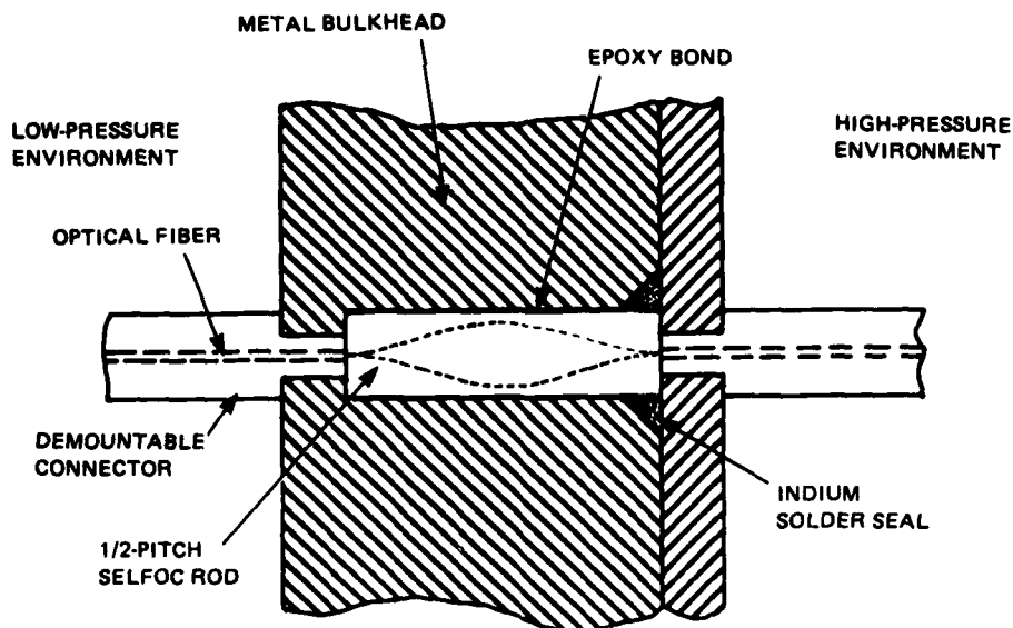
Figure 17. Optical fiber high-pressure penetrator schematic.
