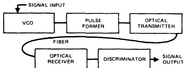
Figure 11. Basic PFM transmission scheme.
