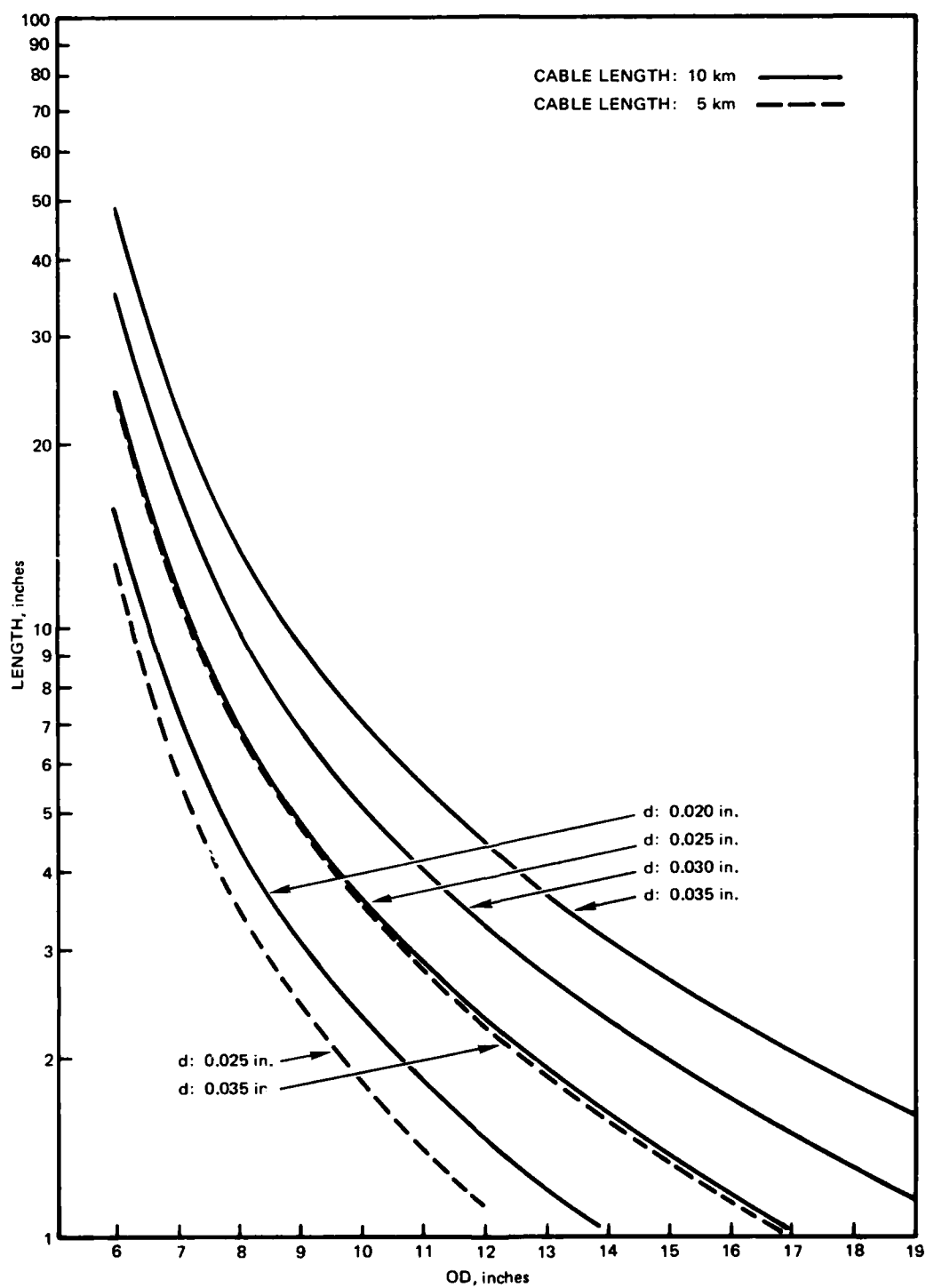
Figure 10. Plot of spool length as a function of OD with an ID of 5 inches and cable lengths of 5 and 10 km.
