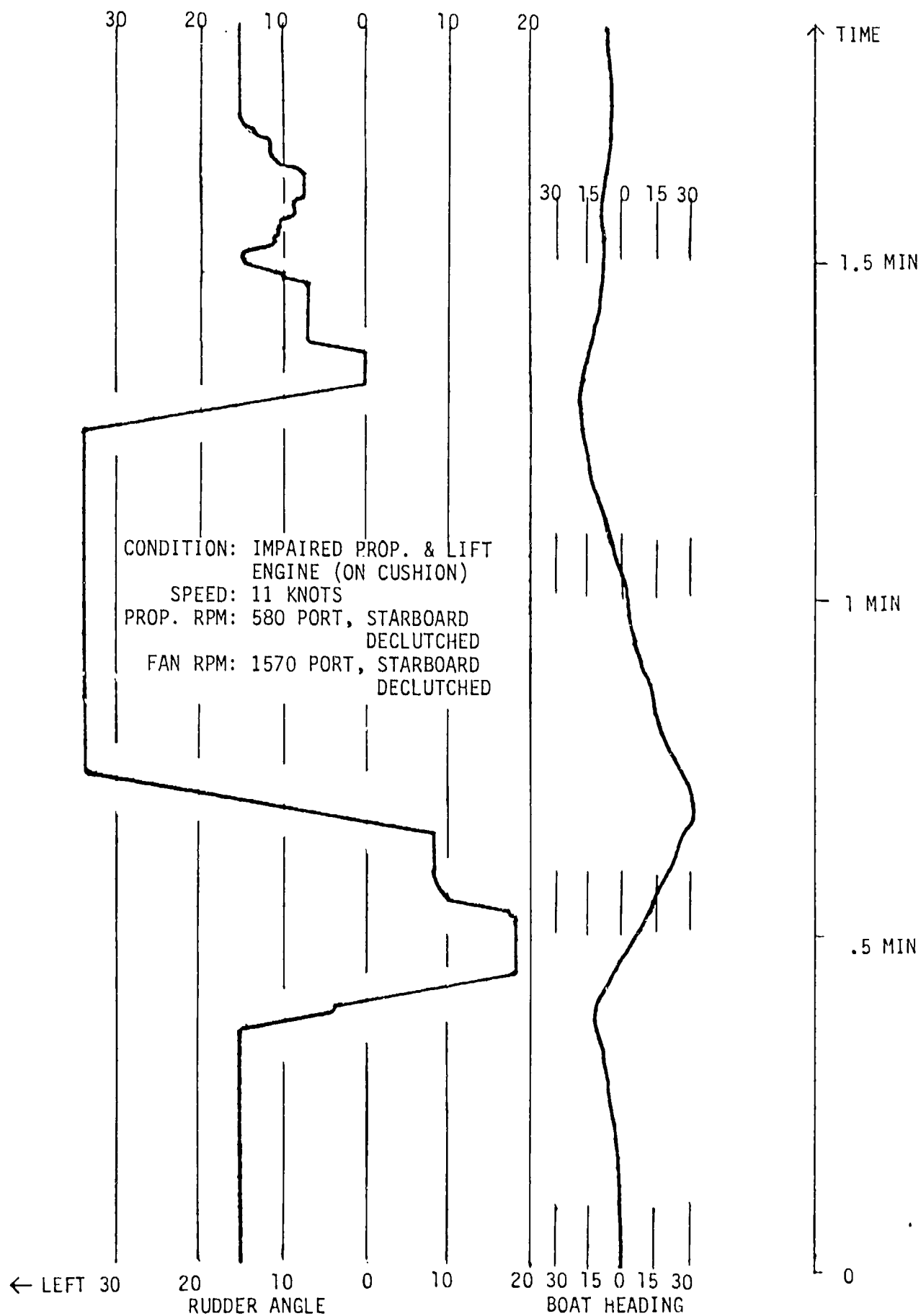
FIGURE 21. DIRECTIONAL STABILITY AT NORMAL LOW SPEED WITH IMPAIRED PROPULSION AND FAN ENGINE (ON CUSHION)
