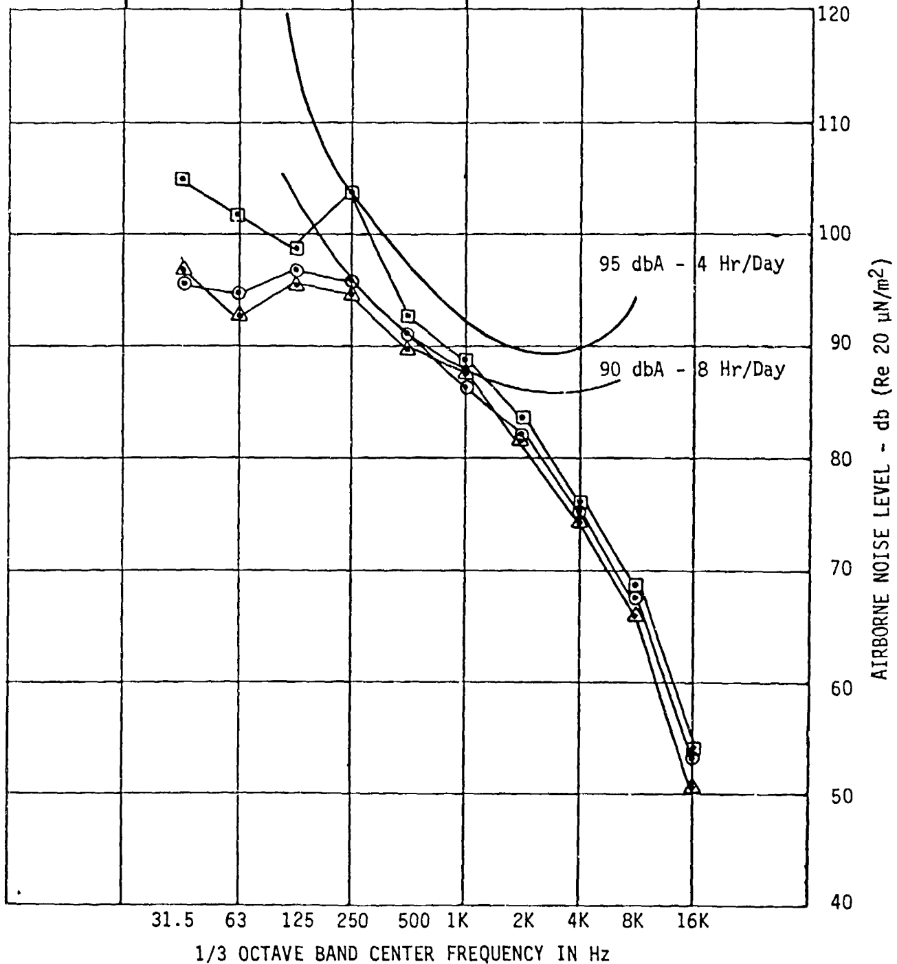
FIGURE 38. AMBIENT NOISE LEVEL - OUTSIDE - CENTER MAIN AFTERDECK
