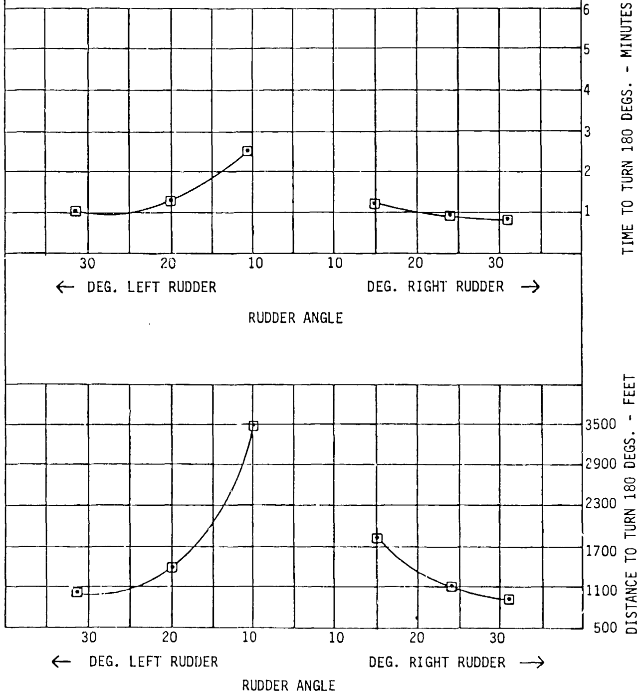
FIGURE 15. TURNING DIAMETER FOR VARIOUS RUDDER ANGLES AND SPEEDS (ON CUSHION) (Continued)
