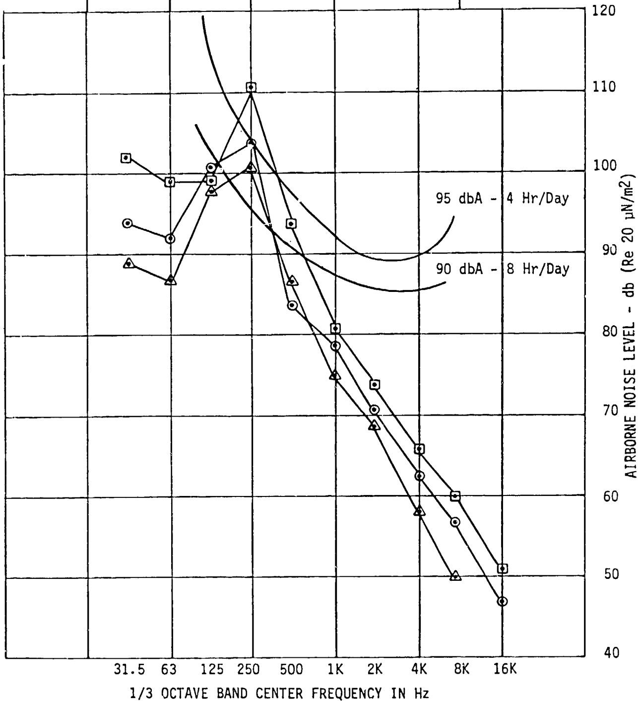
FIGURE 37. AMBIENT NOISE LEVEL - OUTSIDE - MAINDECK - MIDSHIP
