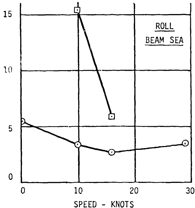
FIGURE 7. COMPARISON OF SEAWORTHINESS RESULTS FOR VARIOUS SEA STATES AND HEADINGS
