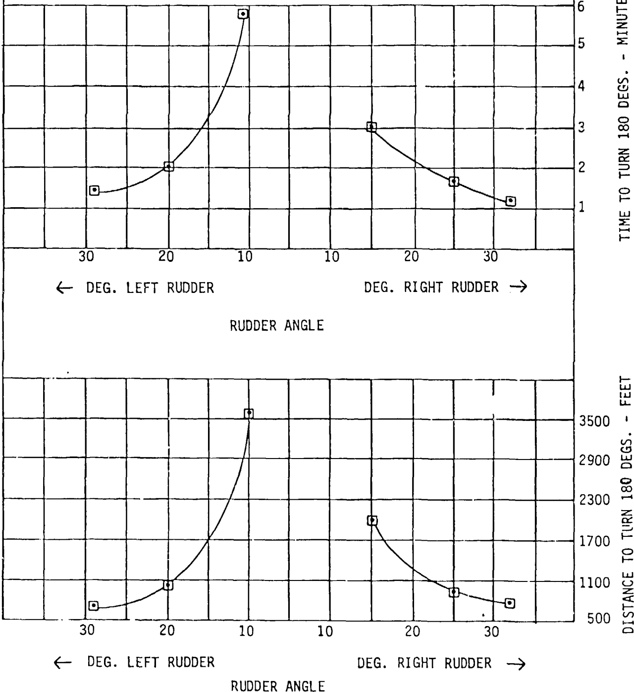
FIGURE 15. TURNING DIAMETER FOR VARIOUS RUDDER ANGLES AND SPEEDS (ON CUSHION)
