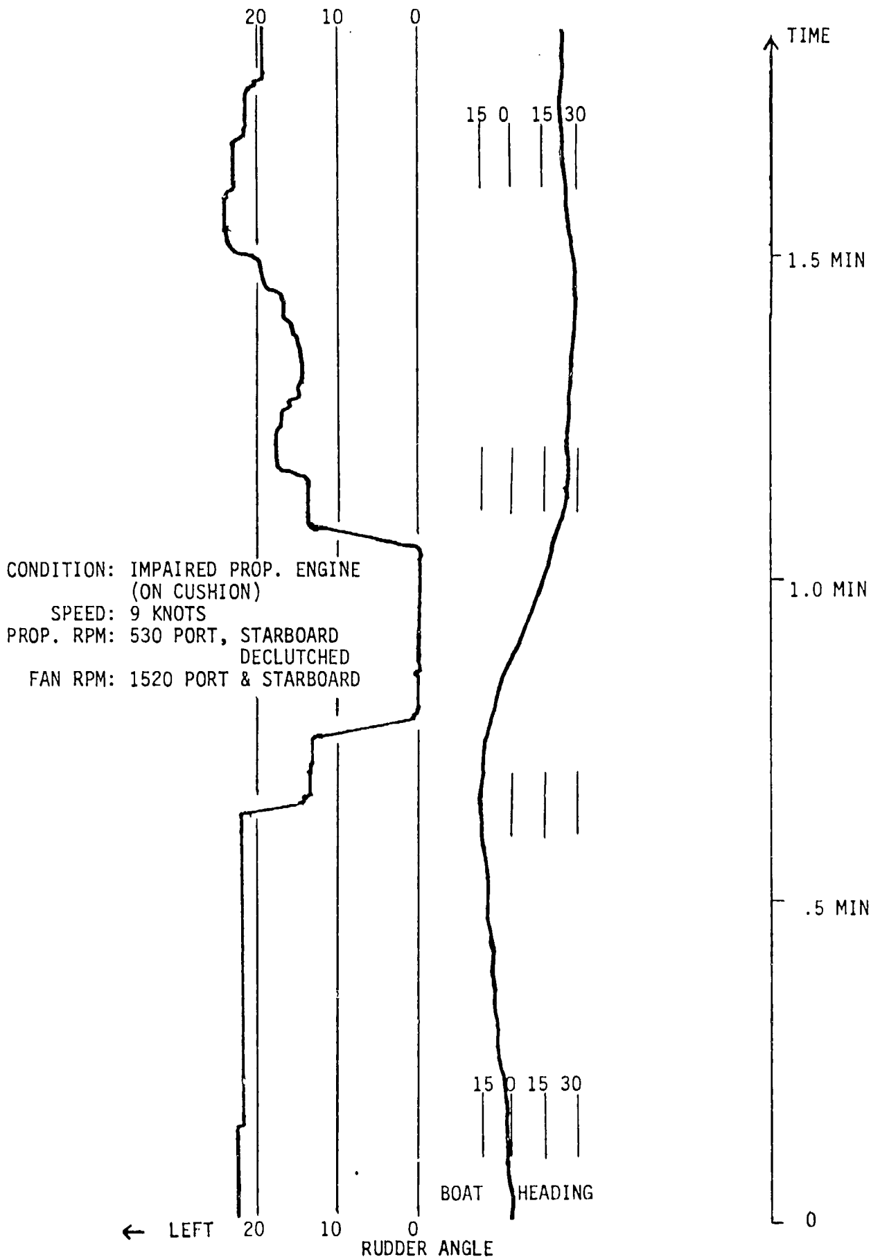
FIGURE 20. DIRECTIONAL STABILITY AT NORMAL LOW SPEED WITH IMPAIRED PROPULSION ENGINE (ON CUSHION)
