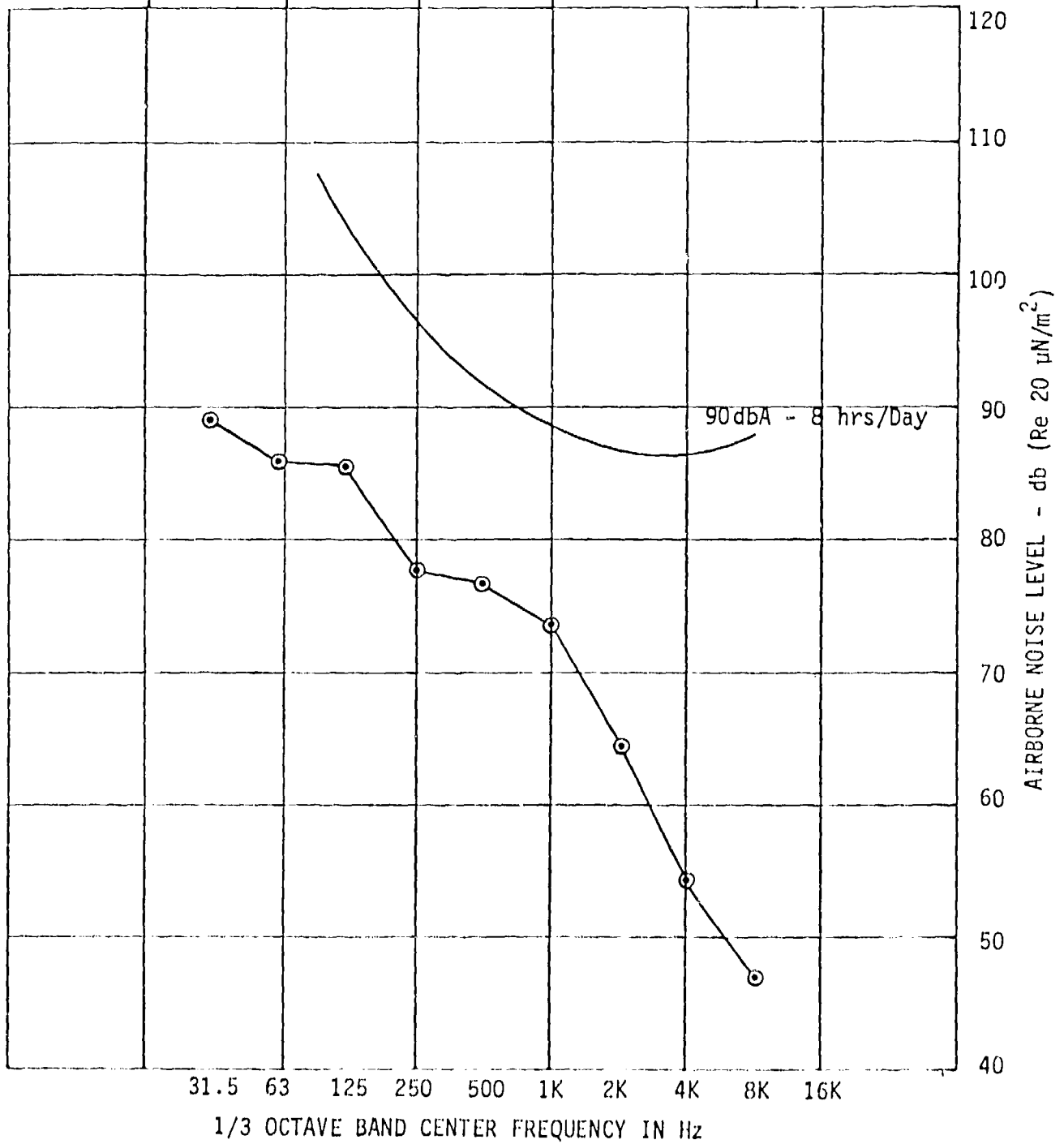
FIGURE 34. AMBIENT NOISE LEVEL - CENTER OF GALLEY AREA - CENTER LINE PASSAGEWAY - DOOR CLOSED
