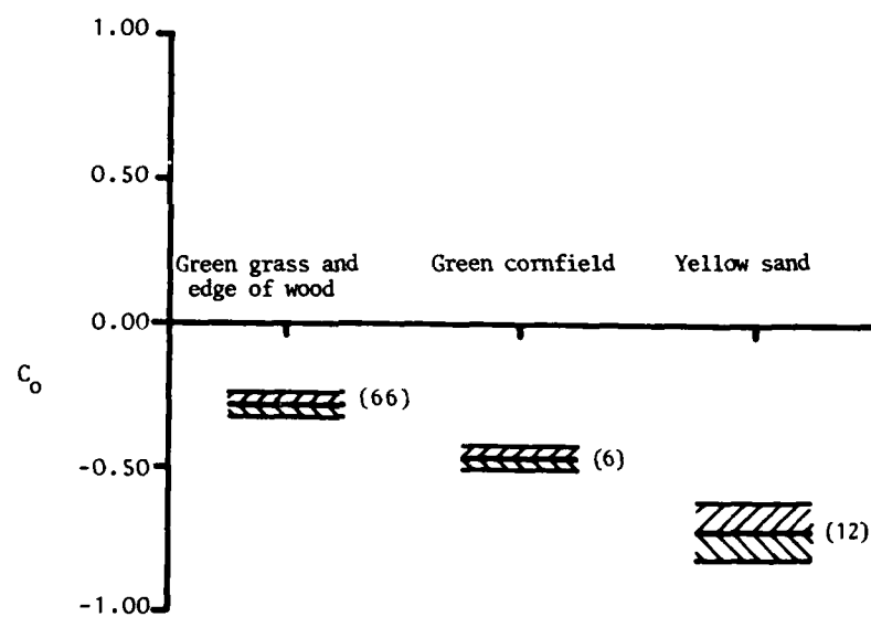
Fig.4 Inherent contrast C_o for various backgrounds. Target area in shadow
