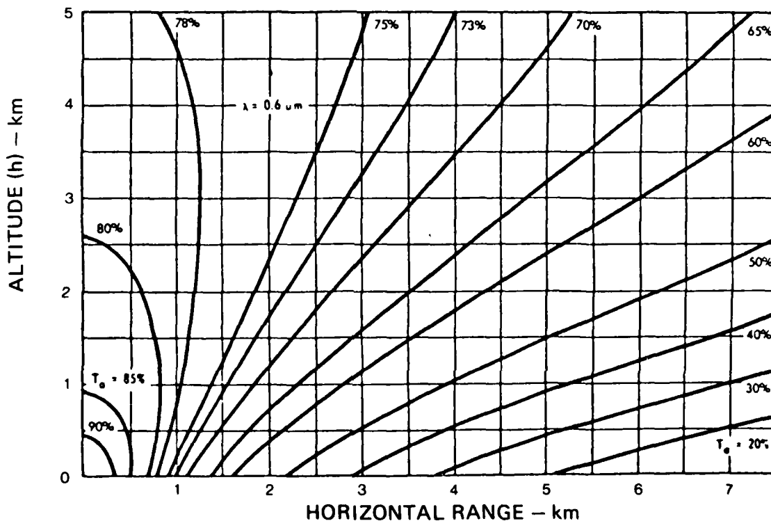
Fig. 6 Contours of constant atmospheric transmittance for radiation at 0,6 \mu\text{m} in a atmosphere-visibility 12 km
