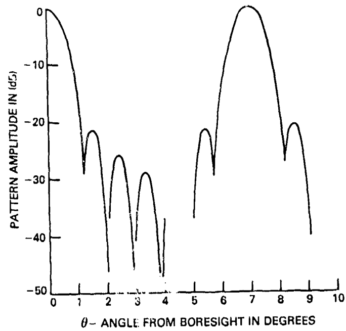
Fig. 16 - Scan plane patterns of bifocal lens with \alpha = 5^\circ
