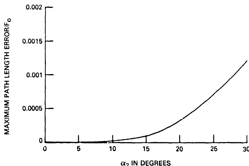
Fig. 15 — Maximum path length error vs \alpha_2 for quadrifocal lens with (F_0/D) = 1
