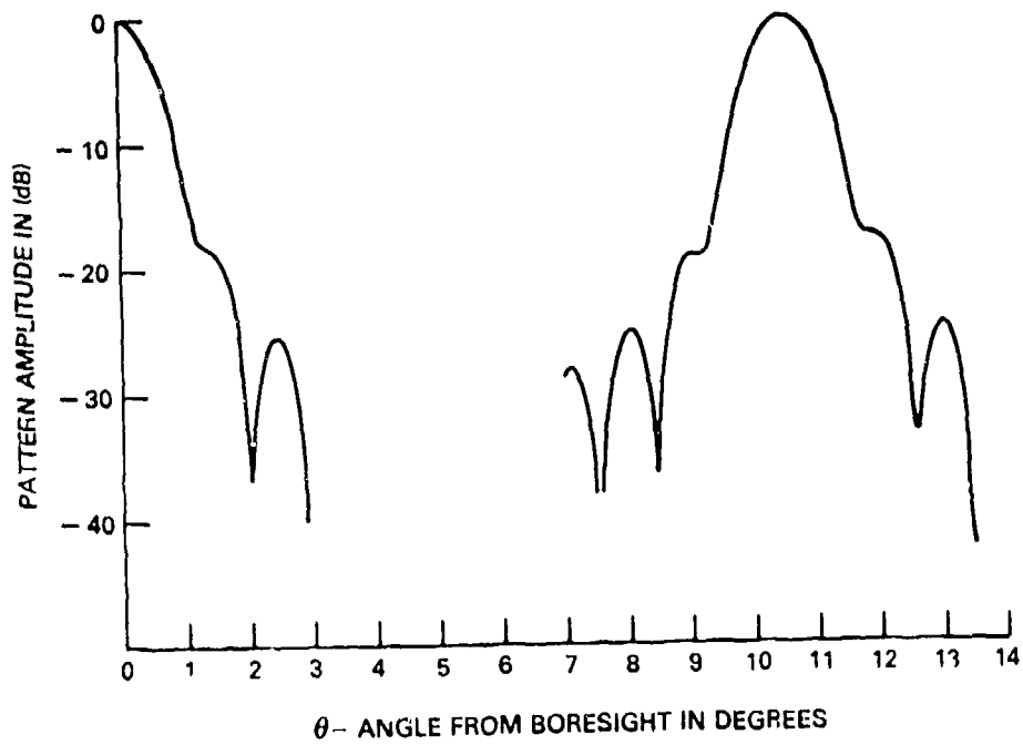
Fig. 17 - Scan plane patterns of bifocal lens with \alpha = 7.5^\circ
