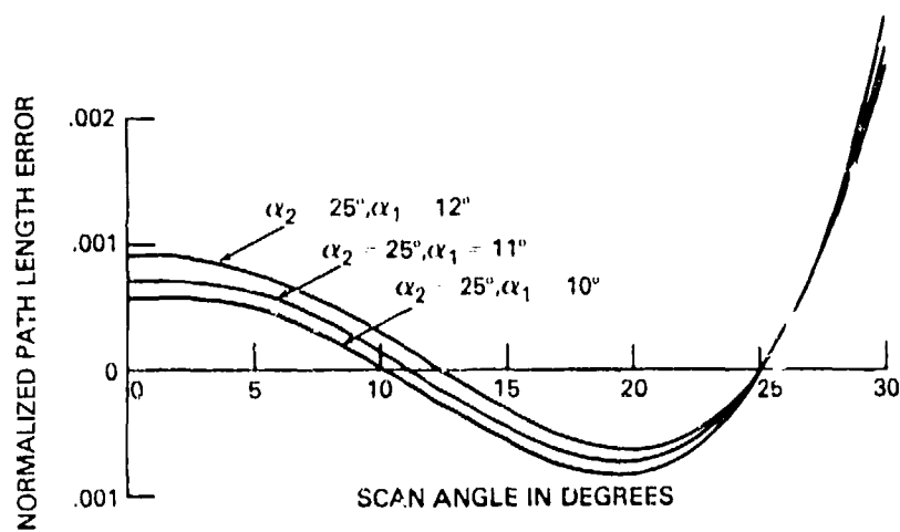
Fig. 14 — Path length error vs scan angle for quadrifocal lens
