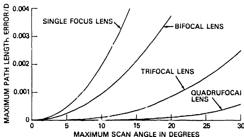
Fig. 15a — Maximum scan angle vs maximum path length error for different lenses
