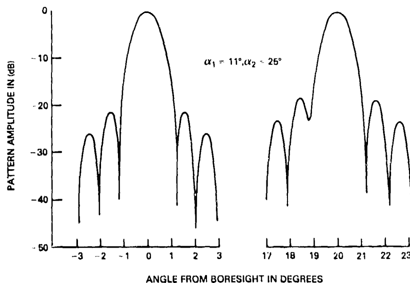
Fig. 20 — Scan plane patterns of quadrifocal lens with feed pattern independent of scan angle
