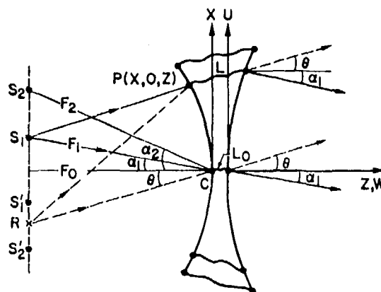
Fig. 11 — Quadrifocal lens geometry in XZ -plane
