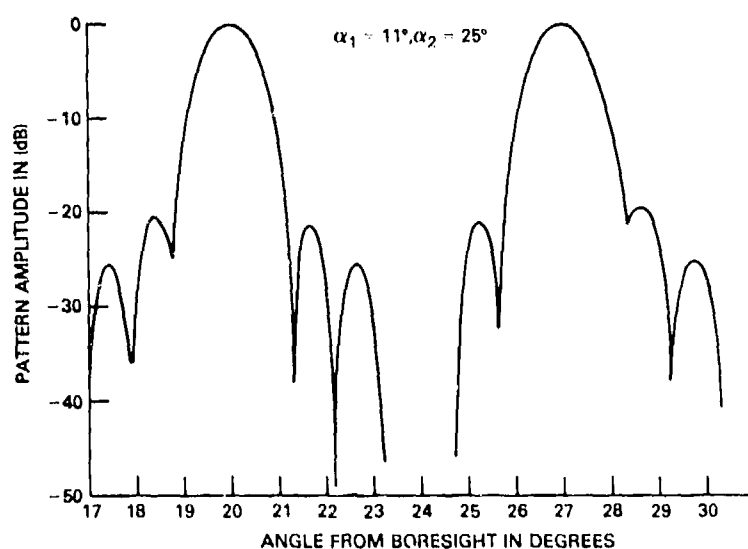
Fig. 21 — Scan plane patterns of quadrifocal lens with feed pattern changed with scan angle
