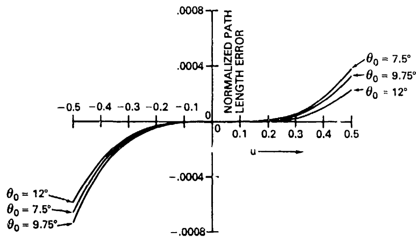
Fig. 8 — Path length errors in XZ -plane for a trifocal lens with \alpha = 15^\circ
