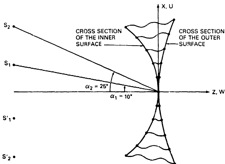
Fig. 12 — Cross section of a quadrifocal lens with \alpha_1 = 10^\circ and \alpha_2 = 25^\circ
