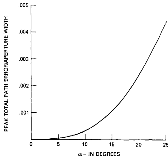
Fig. 10 — Peak total path length error vs \alpha for a trifocal lens with (F_0/D) = 1
