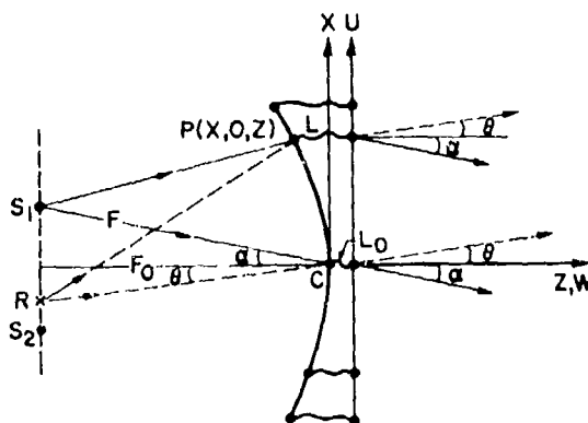
Fig. 1 — Bifocal lens geometry in XZ -plane
