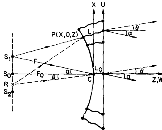
Fig. 6 — Trifocal lens geometry in XZ-plane
