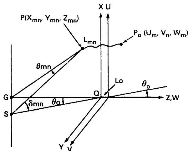
Fig. A1 — Geometry used in determining the amplitude excitation A_{mn}
