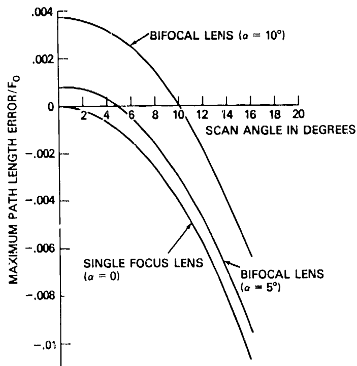
Fig. 4 — Path length error vs scan angle (for u = -0.5 )
