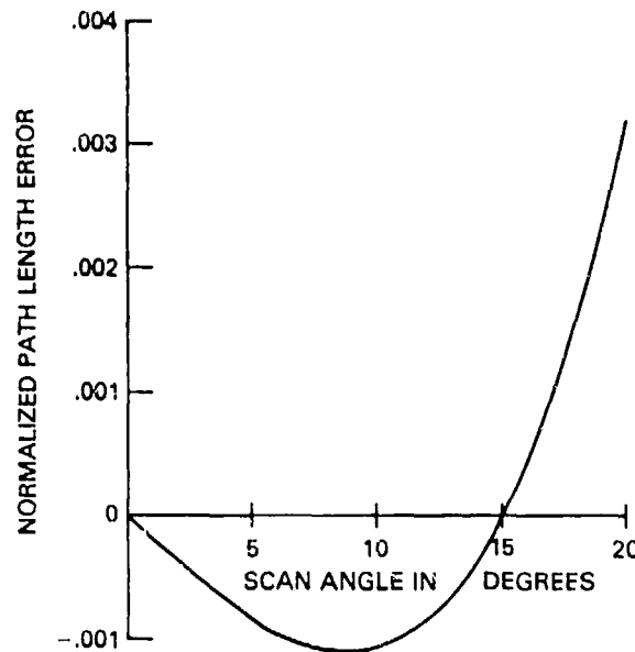
Fig. 9 — Path length error vs scan angle for a trifocal lens ( \alpha = 15^\circ )
