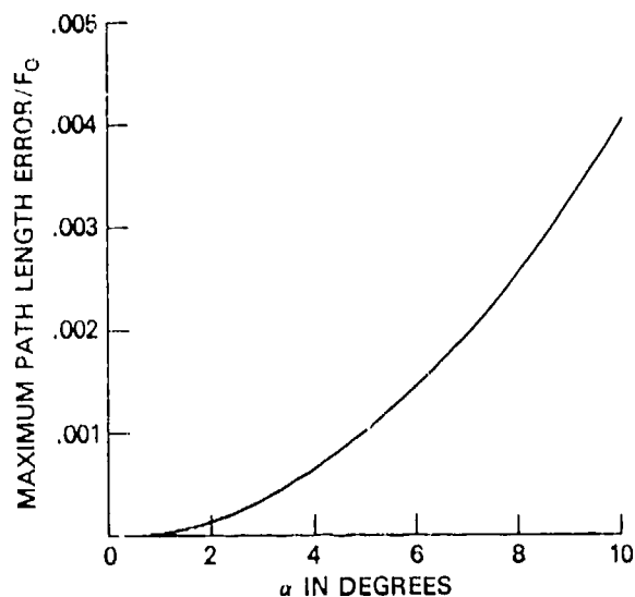
Fig. 5 — Peak path length error vs \alpha for bifocal lens with (F_0/D) = 1
