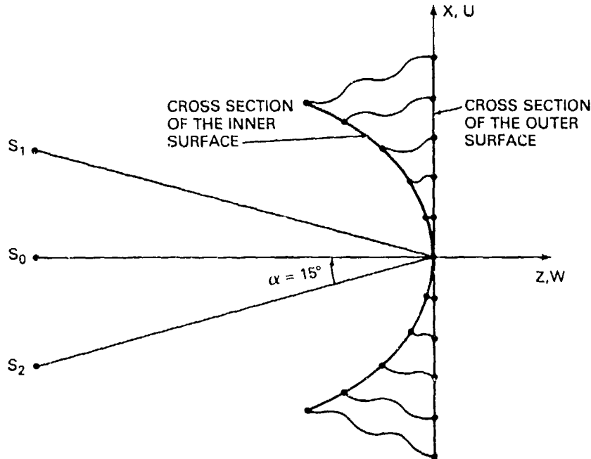
Fig. 7 — Cross section of a trifocal lens in XZ -plane, \alpha = 15^\circ
