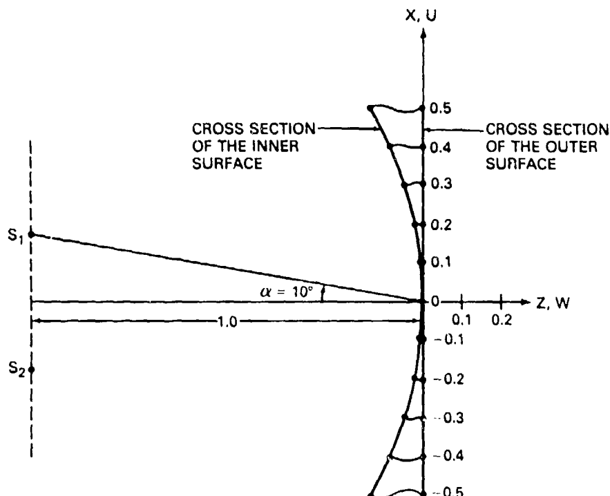
Fig. 2 — Cross section of a bifocal lens in XZ -plane, \alpha = 10^\circ
