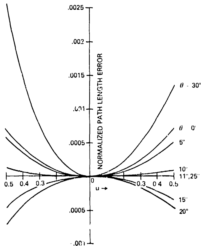
Fig. 13 — Path length errors in XZ-plane for a quadrifocal lens with \alpha_1 = 11^\circ and \alpha_2 = 25^\circ
