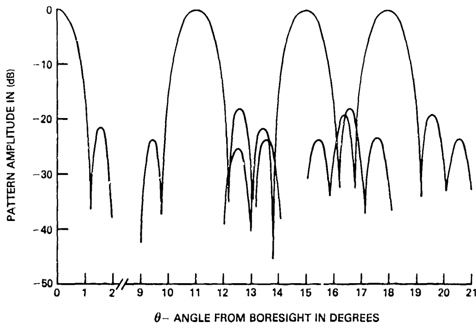
Fig. 18 — Scan plane patterns of trifocal lens with \alpha = 18^\circ
