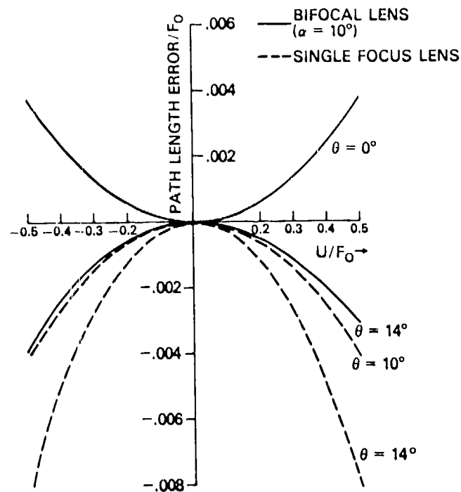
Fig. 3 — Path length errors in XZ-plane
