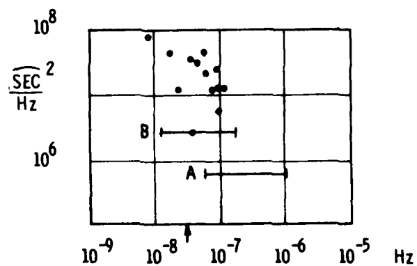
FIG. 4 SPECTRA FROM 10^{-8} - 10^{-6} Hz
