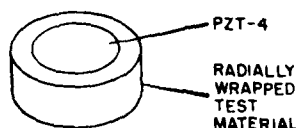
Fig. 7 — Cork-rubber material wrapped radially around ceramic element
