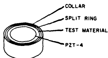
Fig. 5 — Basic configuration of test hydrophone
