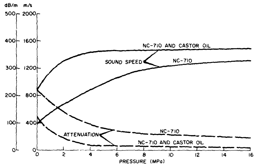
Fig. 26 - Acoustic impedance-tube test results for dry and castor-oil-soaked NC-710
