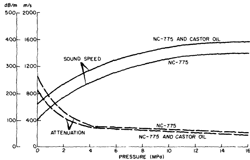
Fig. 27 - Acoustic impedance-tube test results for dry and castor-oil-soaked NC-775
