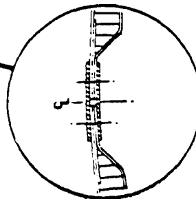
CLAMSHELL JOINT MECHANICAL OR BOND + MECHANICAL
