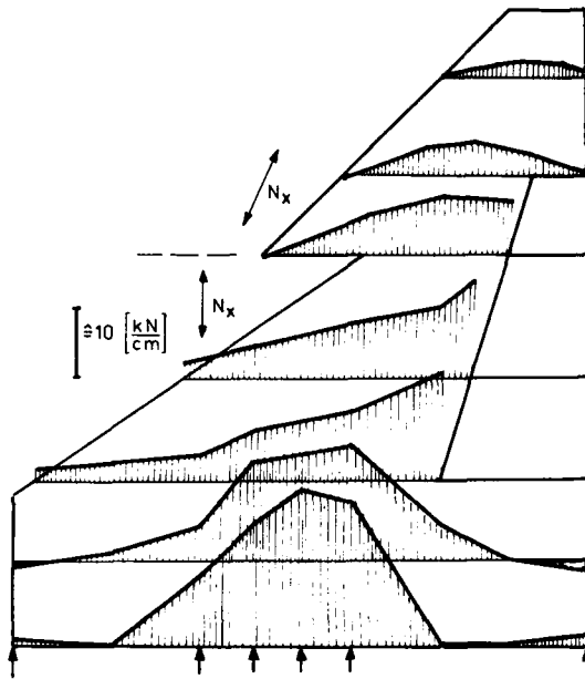
Fig. 23 INTERNAL SKIN LOAD DISTRIBUTION
