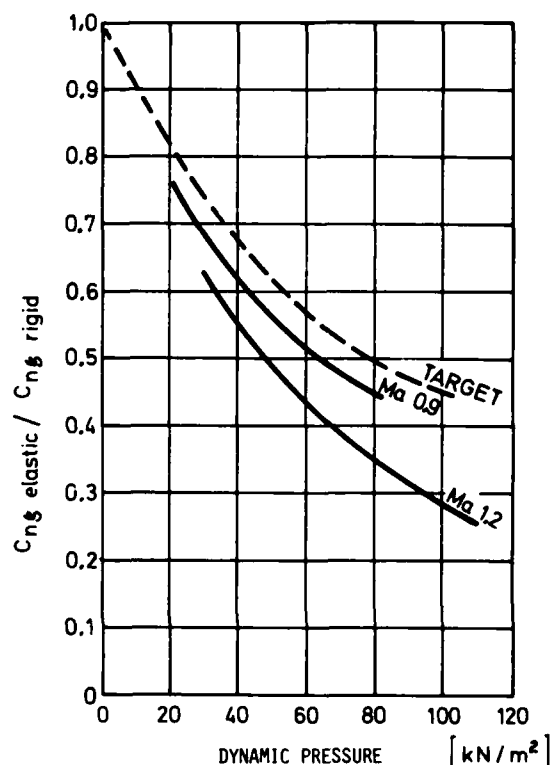
Fig. 17 RUDDER EFFECTIVENESS
