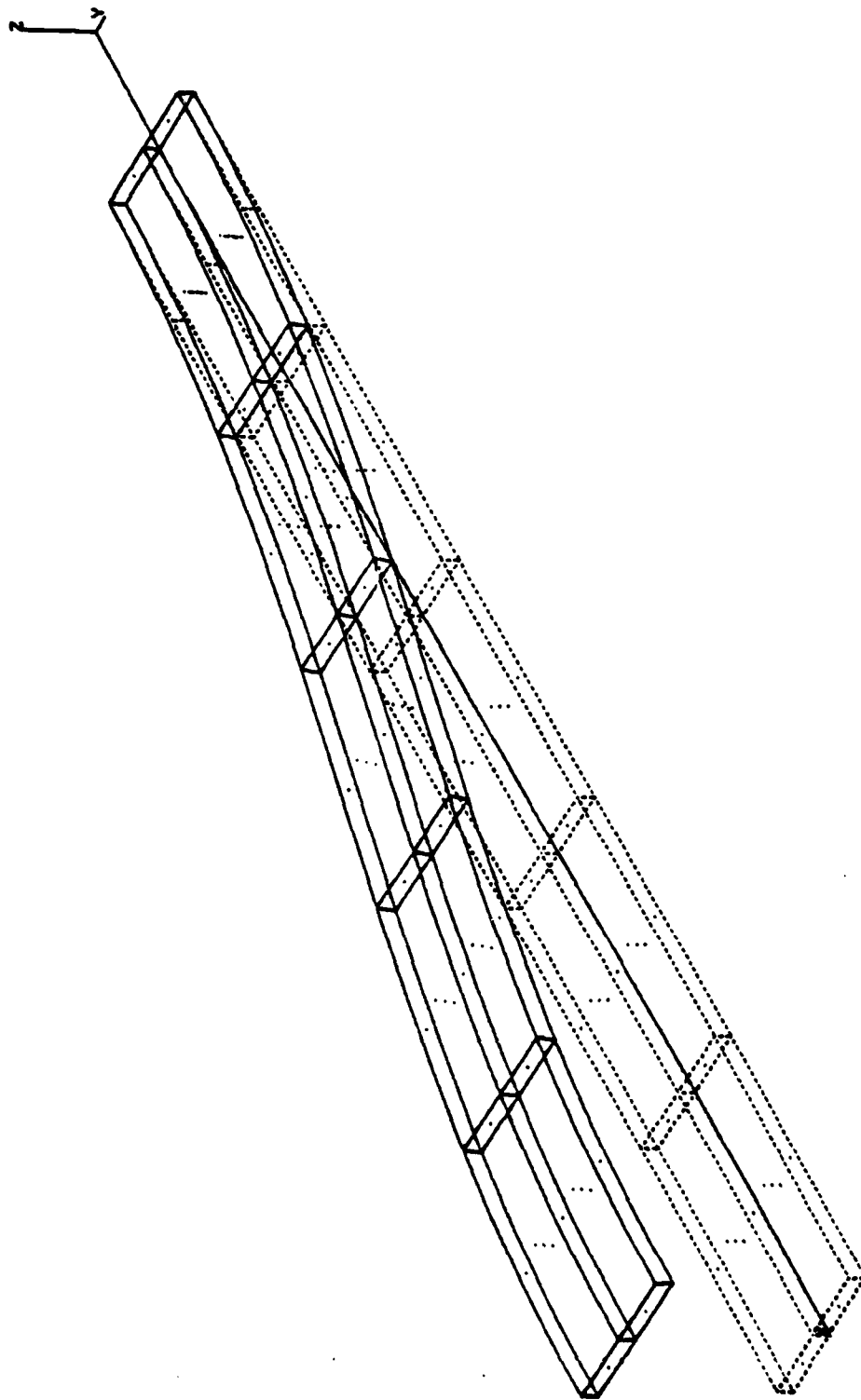
Figure 4.2.14. Plot of deformed and undeformed clamped beam structure illustrating TRANSLATE, ROTATE and REFLECT command. The original structure is illustrated in Figure 4.2.10.
