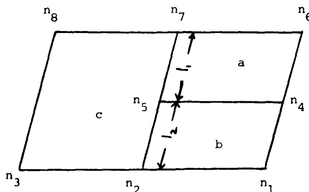
Figure 2.11.6. An example of an incompatible element alignment between elements a, b and c, above. (This is presented in Figure 2.11.5.)
