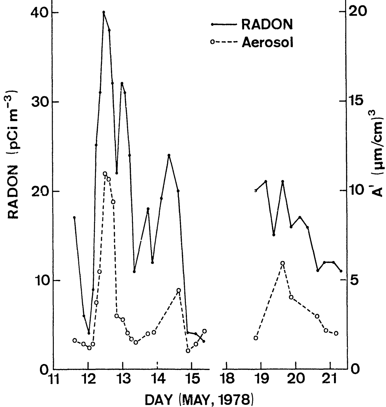
Figure 8. Atmospheric Radon Activity (Solid Line) and Continental Aerosol Coefficient (Dashed Line), During CEWCOM-78.
