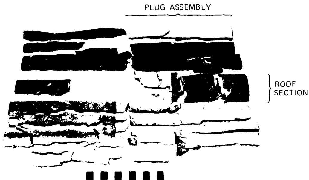
FIGURE 76 TRENCH FRAGMENTS RECOVERED FROM LEAKY PLUG TEST 35
