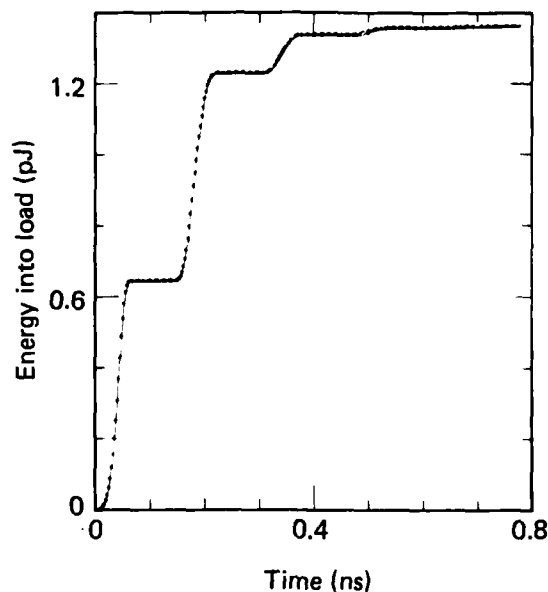
FIG. 8.16. Cumulative energy into a 50\ \Omega load on a 1.13-m monopole for a 5-ns, 1 V/m incident plane wave.
