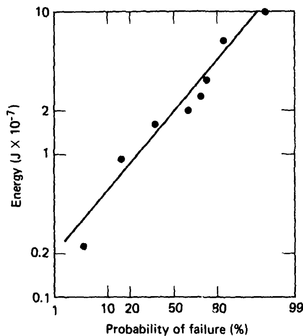
FIG. 8.20. Lognormal probability plot of diode failure data.
