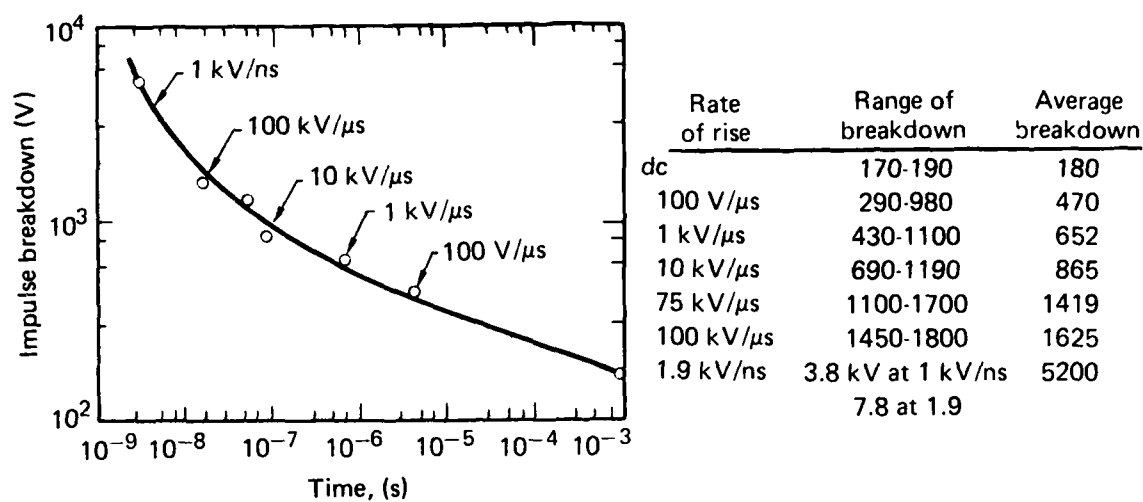
(a) Volt-time curve of one type of spark gap. (Adapted from Hart and Higgins, Joslyn Electronic Systems, Goleta, CA, 1973.)
