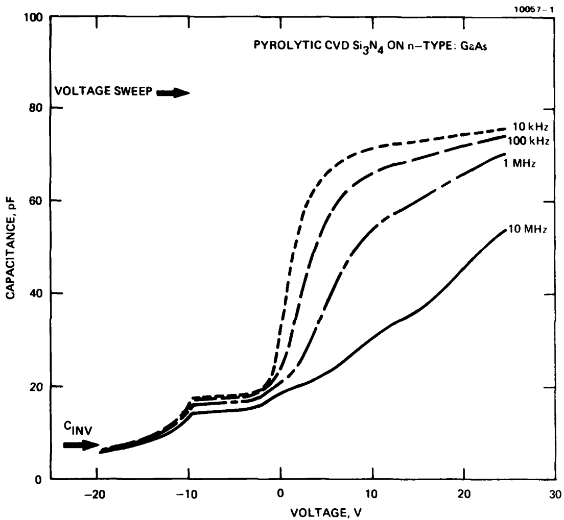
Figure 1. Capacitance of Al-Si 3 N 4 -GaAs structure as a function of test frequency and Al bias voltage.
