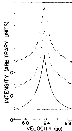
FIG. 1. Spectrum of convoy electrons emergent near 0 \text{ deg} from 16\text{-MeV } \text{O}^{3+} ions traversing a 30\text{-}\mu\text{g}/\text{cm}^2 C foil. The upper data points are obtained from the raw spectrum (lower points), through a correction factor v_e^{-1.6} , to account for the electron-escape-depth velocity dependence estimated from Ref. 11. The lower curves represent respective fitted cusp shapes, which better display the degree of symmetrization produced.
