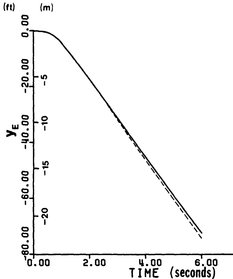
Fig. 2. Lateral deviation of rocket center of mass, y_E , for \alpha_y = 0.001 .
