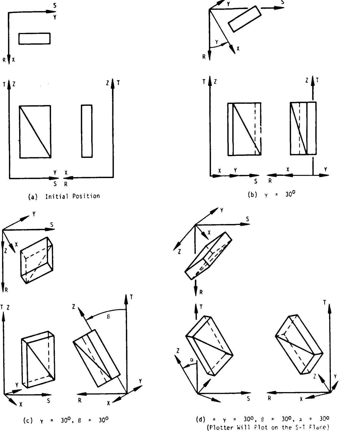
Figure 2. Plotter - model orientation.
