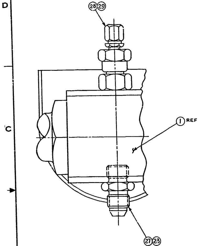
VIEW C-C
