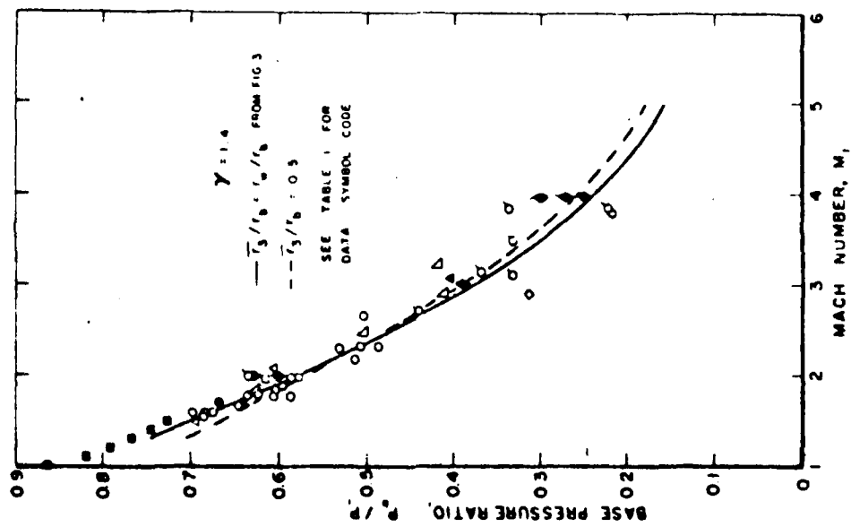
Figure IV-15. Axisymmetric Supersonic Base Pressure From Modified Conical Pressure Rise Method
