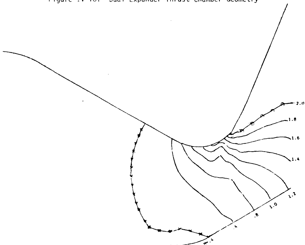
Figure IV-19. Annular Nozzle Throat Section Mach No. Contours
