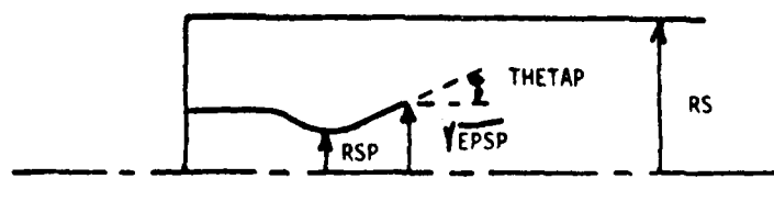
Figure 1. Nozzle Geometry for Option 1
