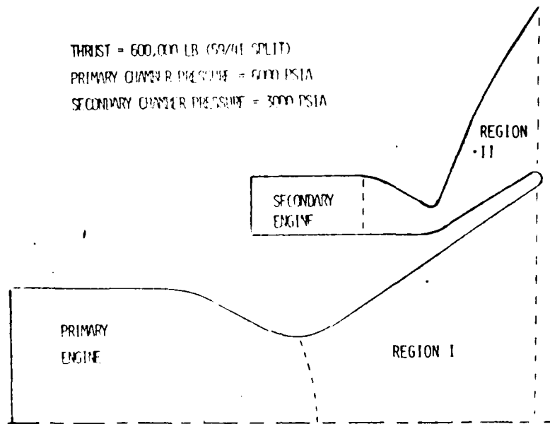
Figure IV-18. Dual Expander Thrust Chamber Geometry
