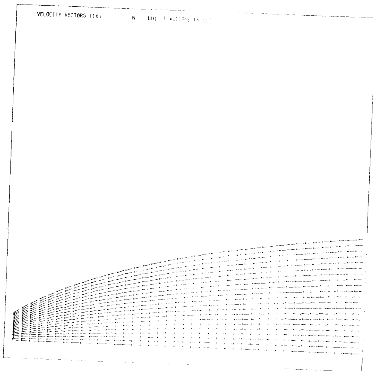
Figure III-17. Conventional Nozzle Downstream Velocity Vector Plot
