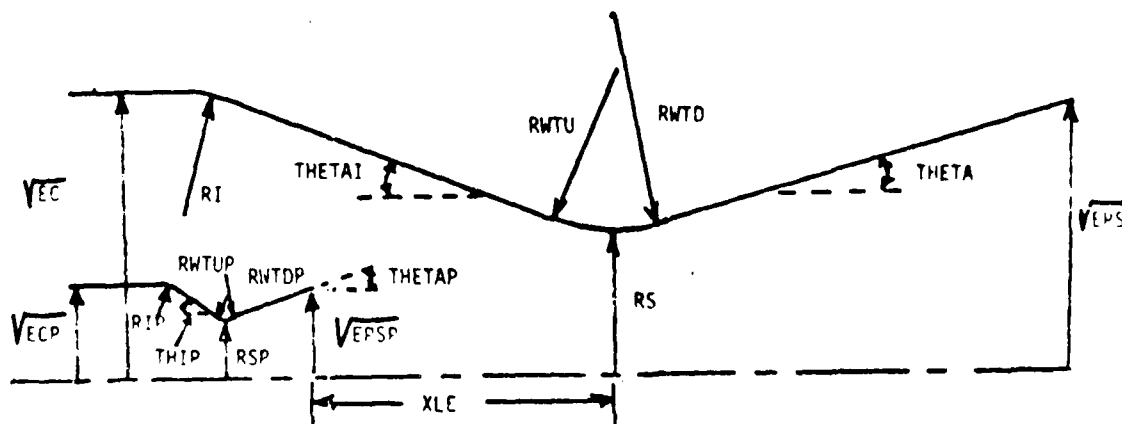
Figure 2. Nozzle Geometry for Option 2
