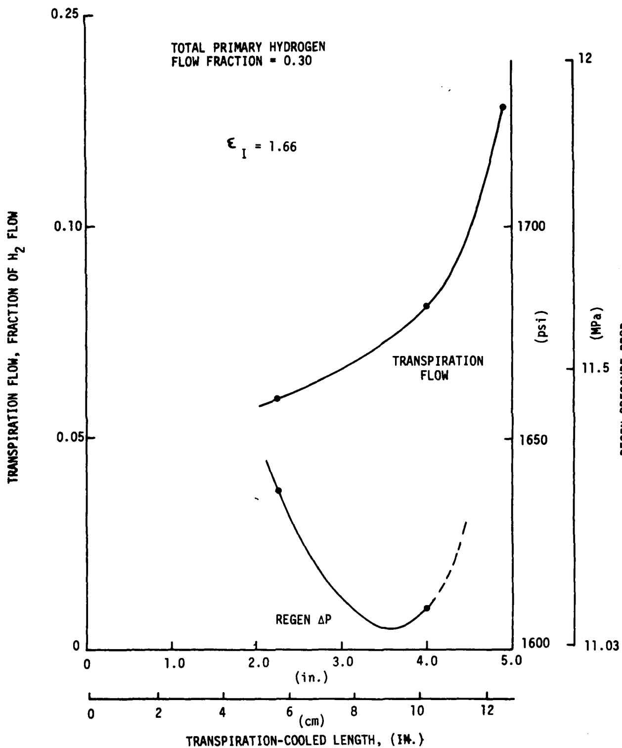
Figure V-18. Dual Expander Transpiration Cooling
