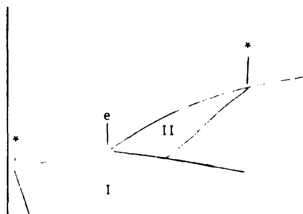
c. REGIONS
