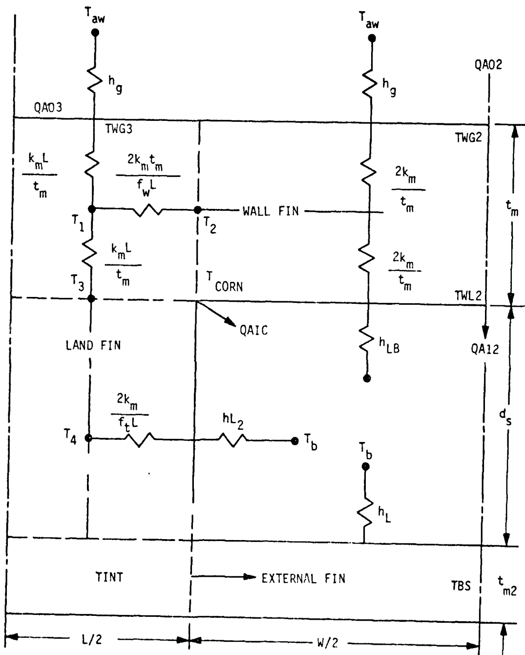
Figure V-9. Schematic of Wall Conduction Model
