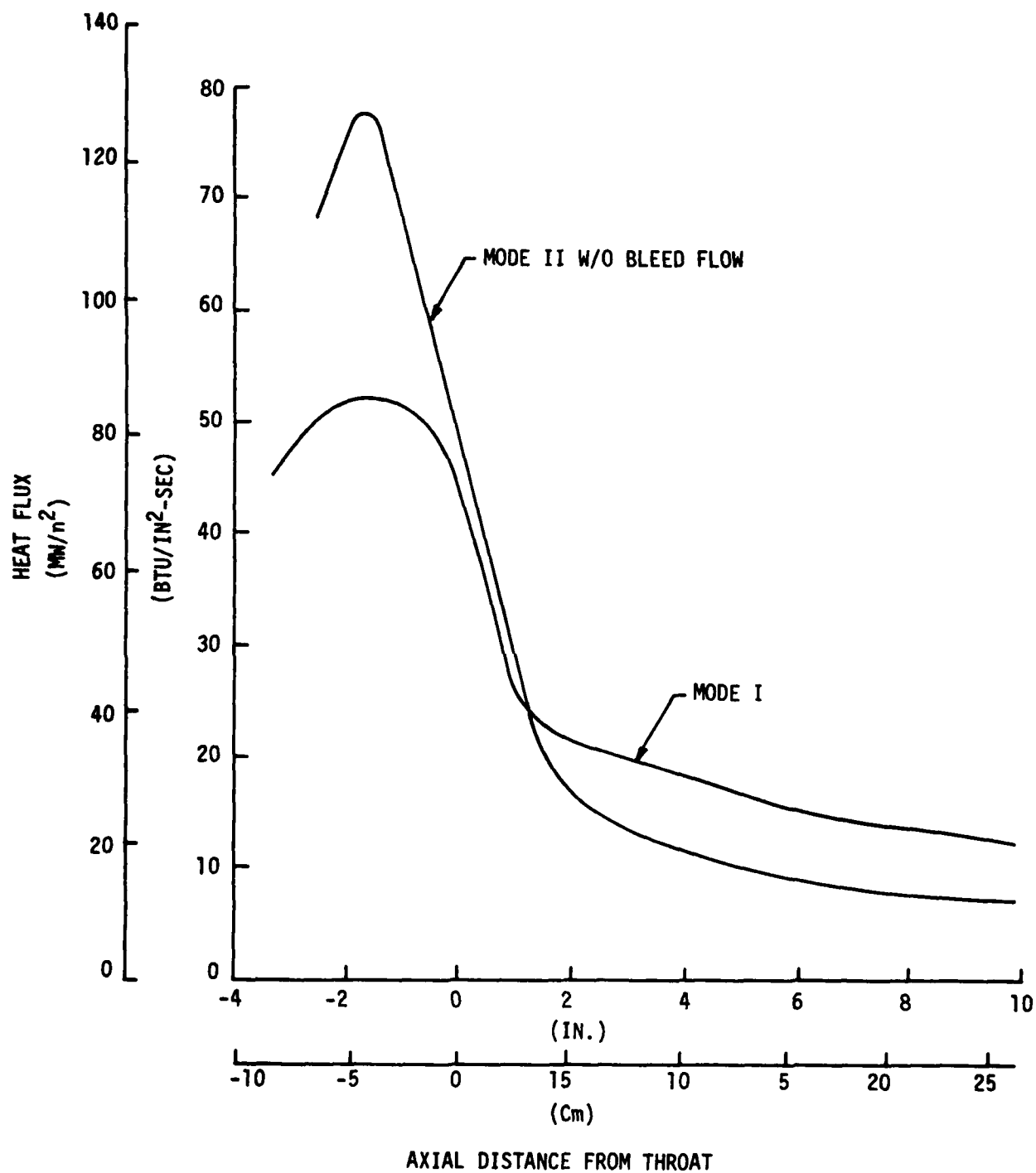
Figure V-13. Comparison of Secondary Throat Region Heat Fluxes
