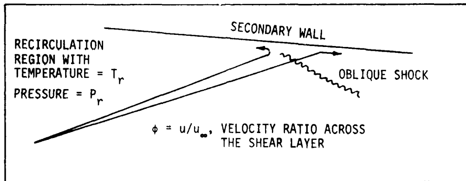
Figure III-2. Shear Layer Streamlines and Velocity Profile
