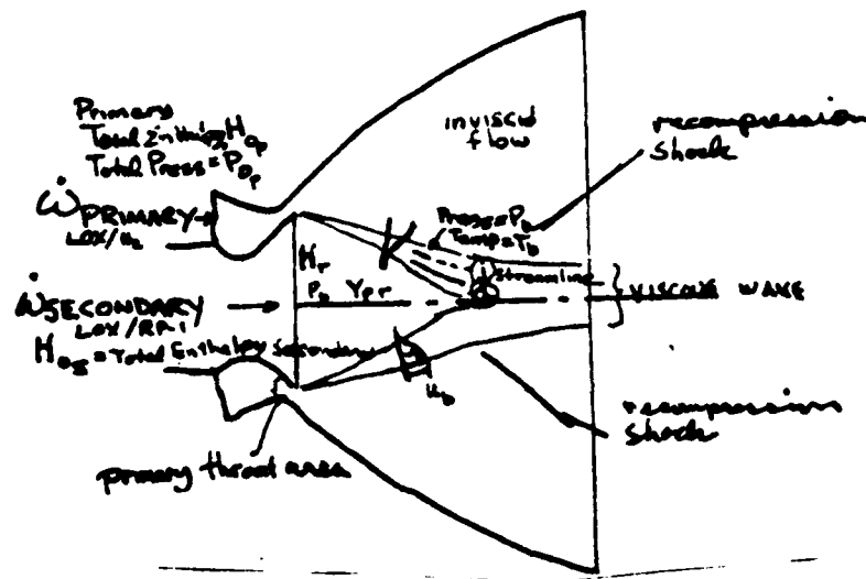
Figure 1. Dual Expander Engine
