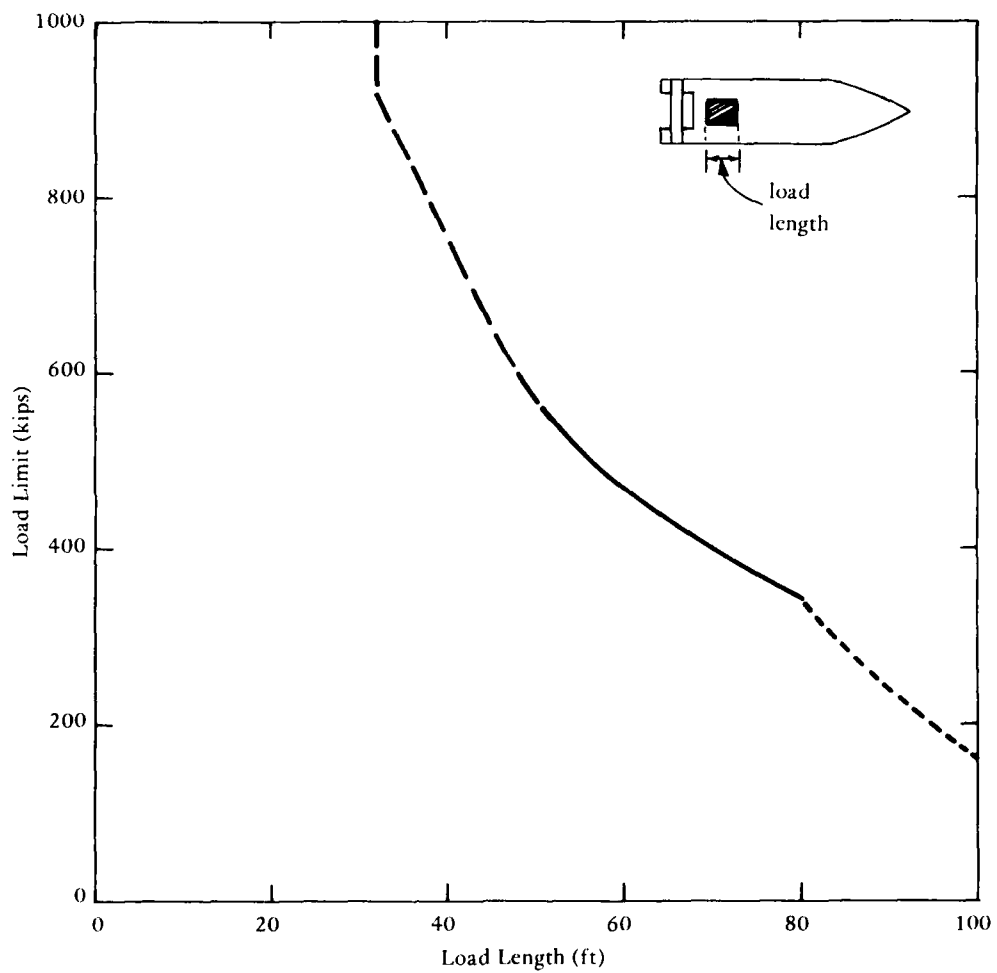
Figure 10. Projected LASH lighter crane lift capacity for outsized loads.
