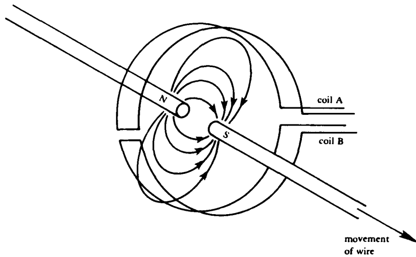
Figure 6. Search coils pick up radial component of flux leakage.
