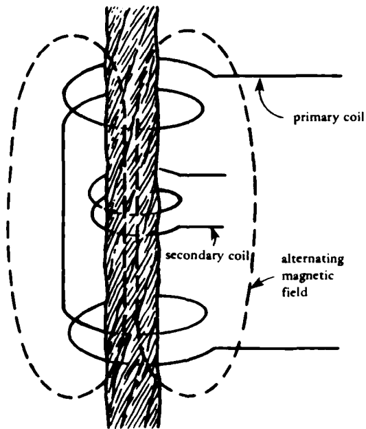
Figure 7. The basic principle of the AC method.
