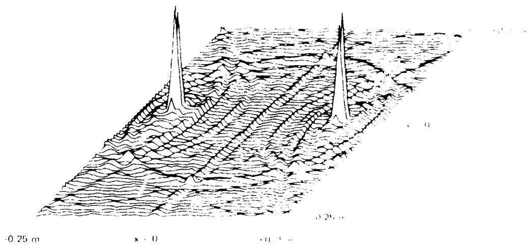
Figure 4-33 Intensity of Image Reconstructed From Magnitude Superposition of Five Existed Images ( \lambda = 0.06\text{ m} )
