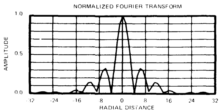
Figure A-5 Annular Spectrum With \cos^{1/2}(\cdot) Tapered Weighting.
