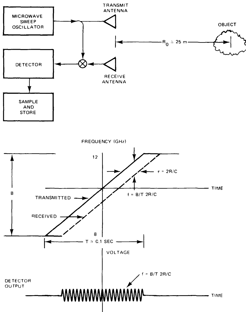
Figure 3-2. Linear-FM Microwave System Instrumentation.
