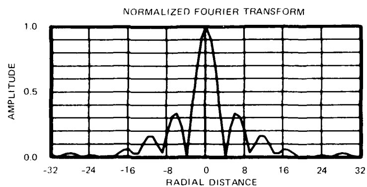
Figure A-7. Annular Spectrum With \cos^2(\cdot) Tapered Edge Weighting.
