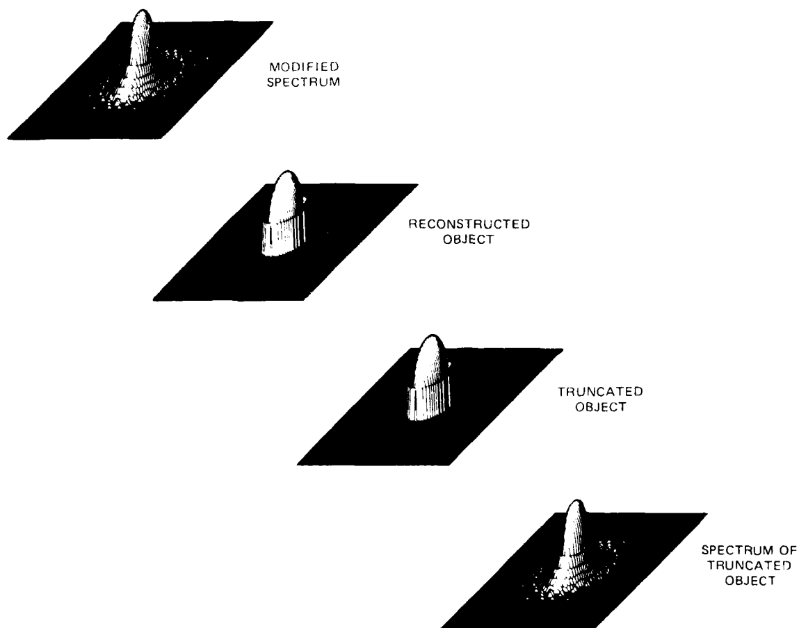
Figure 5-8. Spatial and Spectral Responses for Tenth Iteration of the Algorithm Applied to a Partial Spectrum of a Disc Object (Radius of Object Truncation = 2\lambda ).
