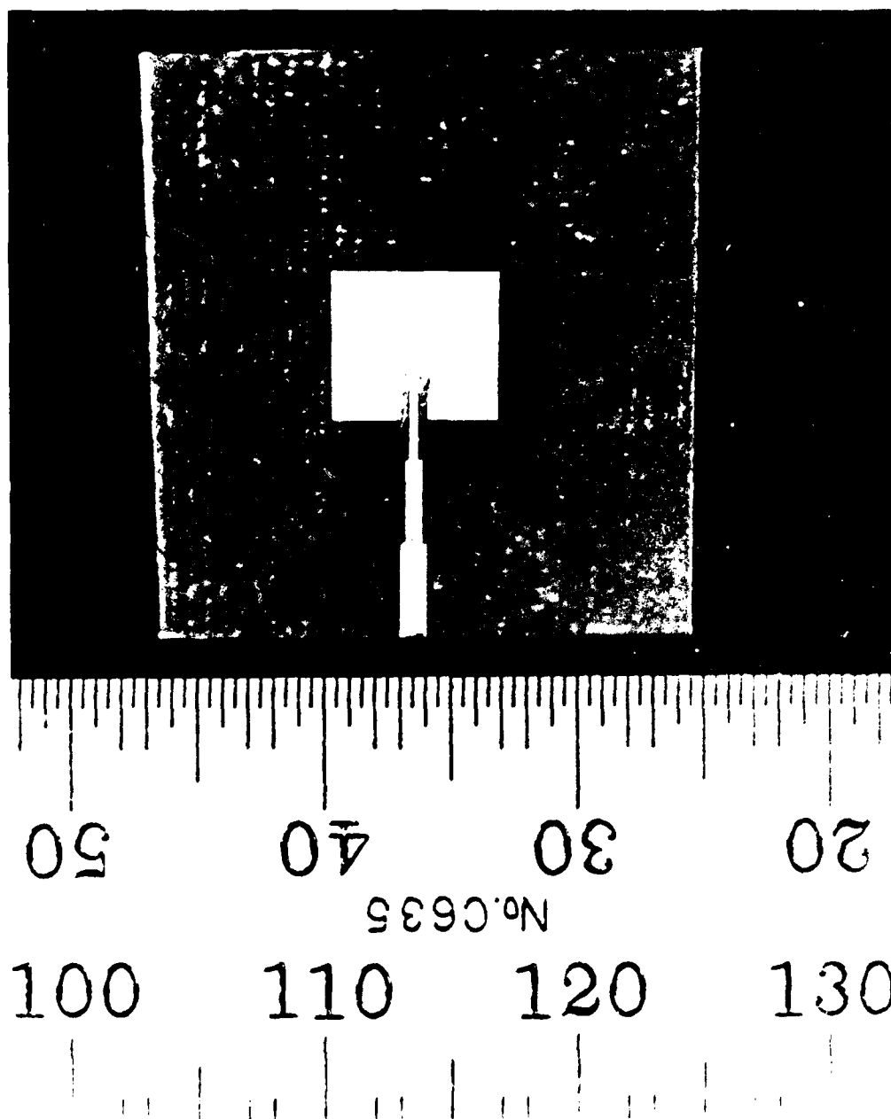
Figure 7. Teflon-Fiberglass Element
