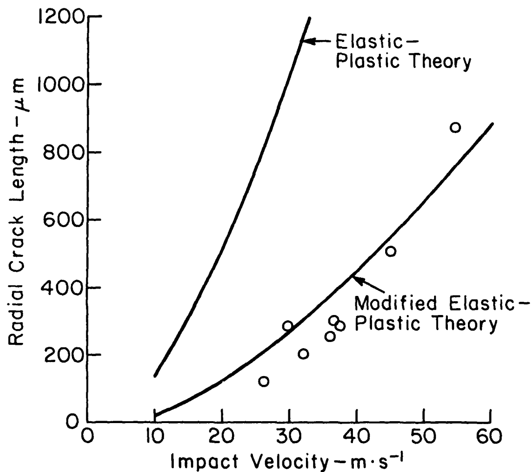
Figure 2. Radial crack length vs. impact velocity for the elastic-plastic theory and the modified elastic-plastic theory based on equations (10) and (11). (As-fired, \text{TP-SrO}_2 ; 1.59 mm diameter tungsten particle spheres).
