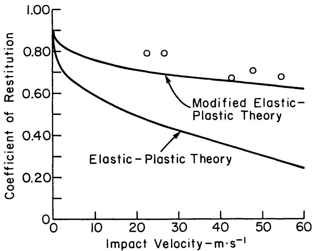
Figure 2b. Comparison of two theoretical coefficient of restitution vs. impact velocity curves with experimental data (under-sized TT-001, 1.59 mm diameter tungsten carbide spheres).
