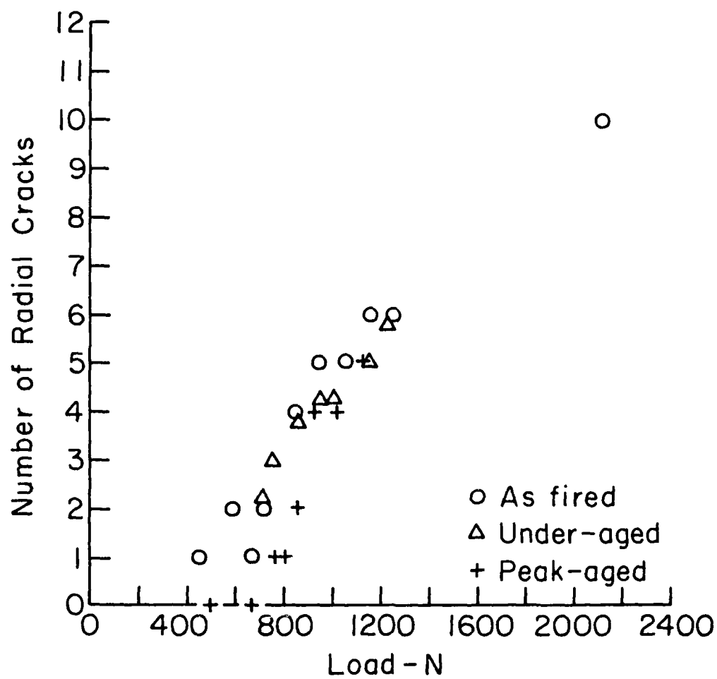
Figure 24 Number of radial cracks vs. load for three aging treatments of TT-ZrO 2 yielding different K_{Ic} values (1.50 mm diameter tungsten carbide spheres).
