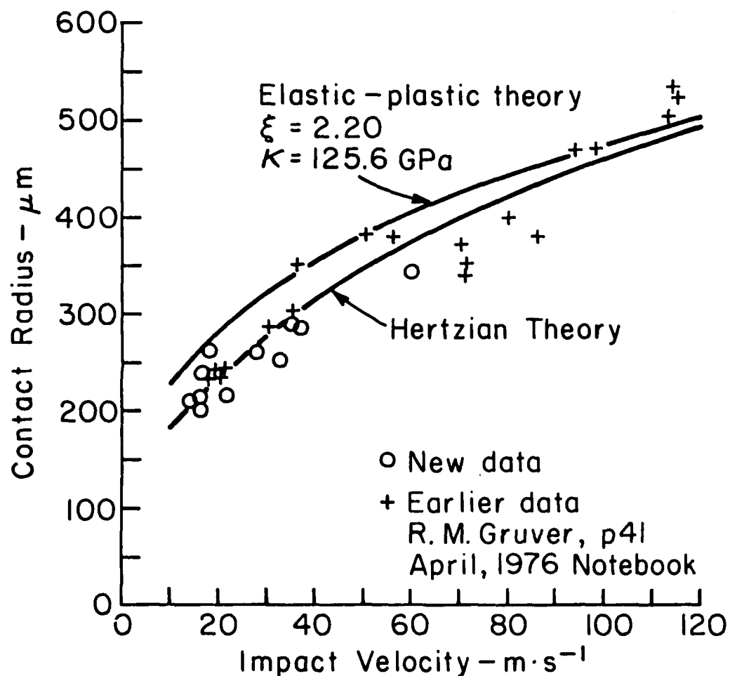
Figure 4 Comparison of theoretical impact contact radii for elastic-plastic and elasticity (Hertzian) theories (china platen, 3 mm diameter glass spheres).
