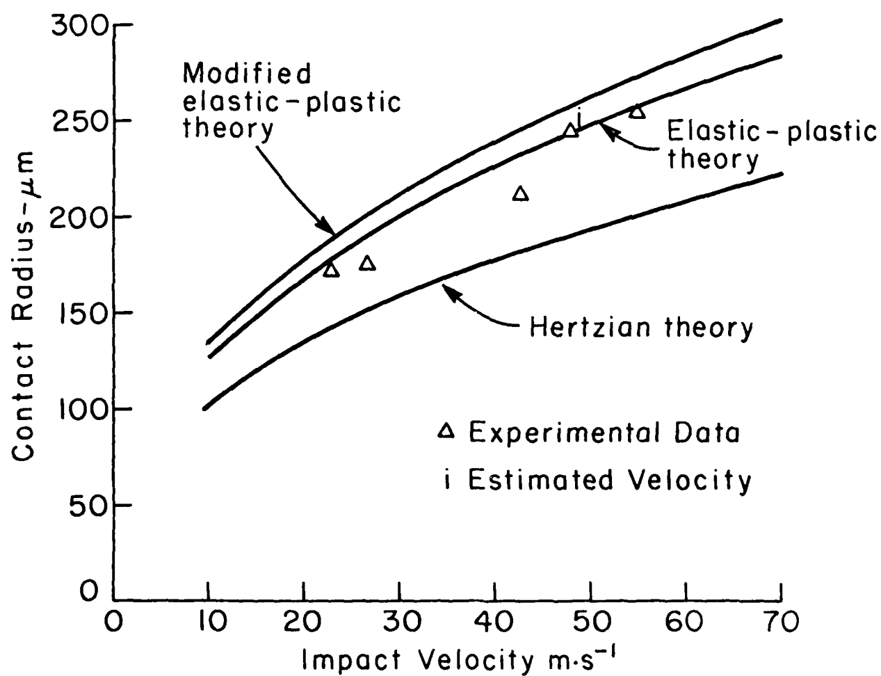
Figure 15. Contact radius vs. impact velocity (under-aged Ti-6Al-4V, 1.5 \mu\text{m} diameter tungsten carbide spheres).
