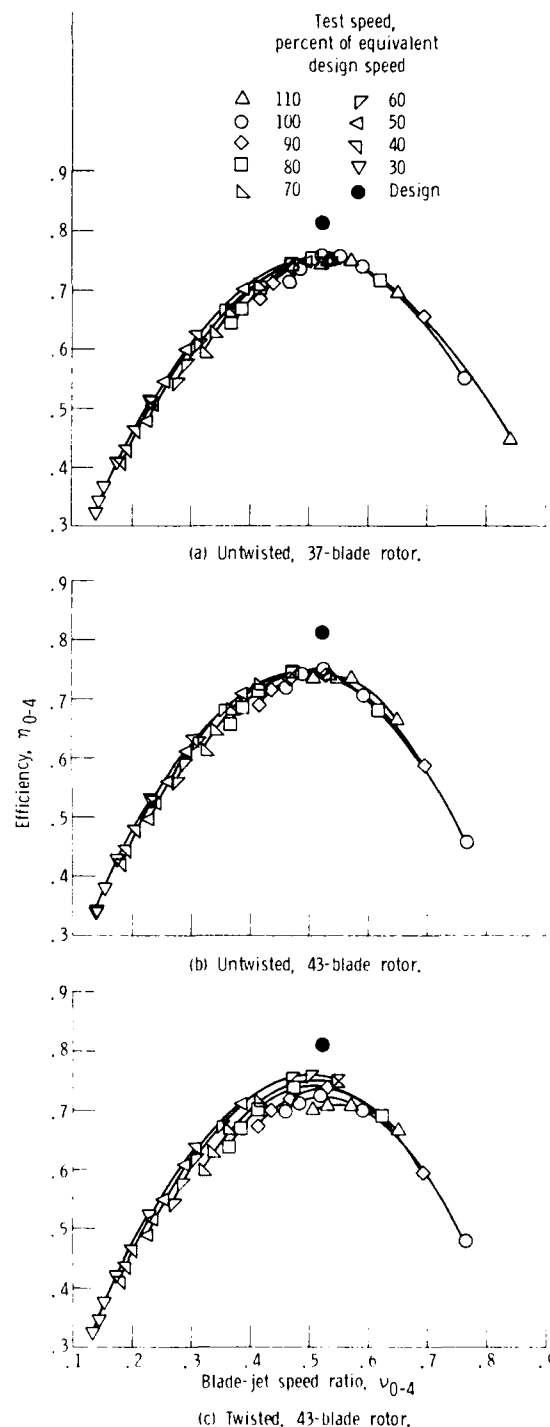
Figure 15. - Variation of efficiency with blade-jet speed ratio with exit diffuser duct installed and with open honeycomb shroud.
