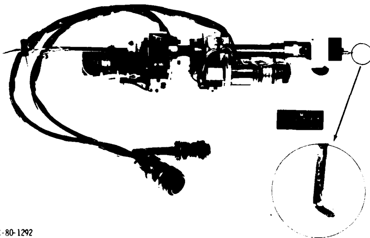
Figure 9. - Rotor exit survey probe and actuator.
