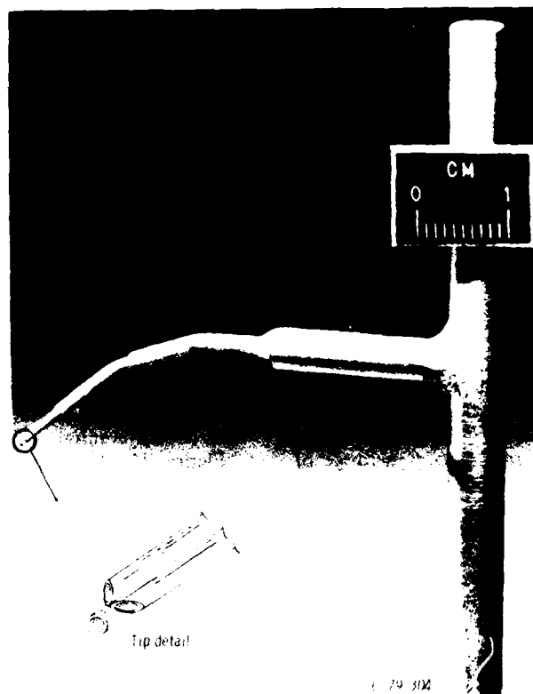
Figure 10. - Stator exit survey probe.
