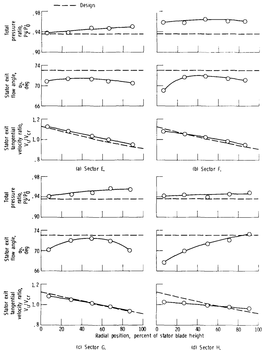
Figure 13. - Stator exit survey results.
