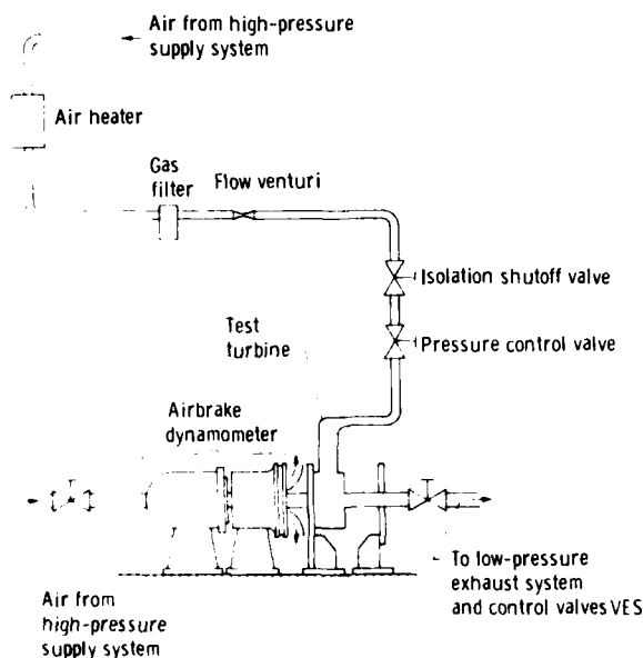
Figure 6. - Experimental equipment schematic.
