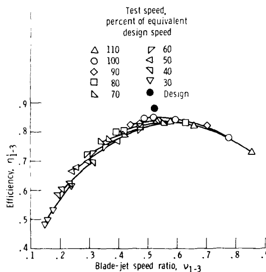
Figure 20. - Variation of efficiency with blade-jet speed ratio with half-depth honeycomb shroud installed - untwisted, 37-blade rotor configuration.
