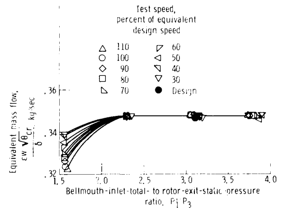
Figure 14. - Variation of mass flow with pressure ratio.
