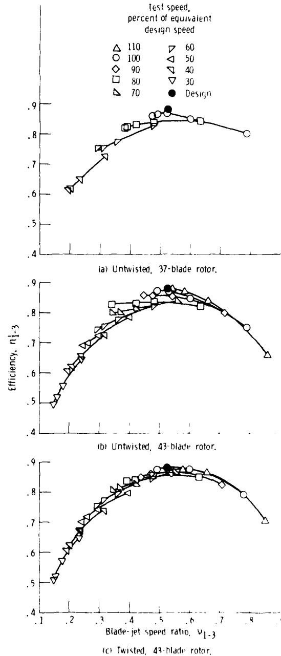
Figure 17. - Variation of efficiency with blade-jet speed ratio with constant-area exhaust duct installed and honeycomb shroud filled.
