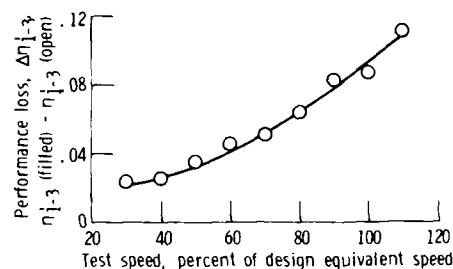
Figure 19. - Performance loss between filled and open honeycomb shroud configurations for untwisted, 43-blade rotor at design blade-jet speed ratio.
