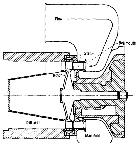
Figure 1. - Turbine cross-sectional schematic.
