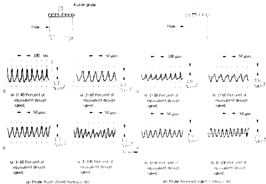
Figure 22. - Results of tests with pressure probe installed in honeycomb shroud of untwisted, 43 blade rotor.
