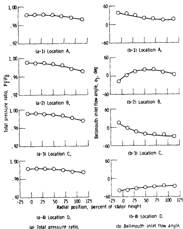
Figure 12. - Bellmouth inlet survey results.
