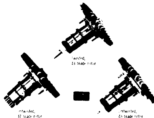
Figure 4. - Rotor configurations tested.
