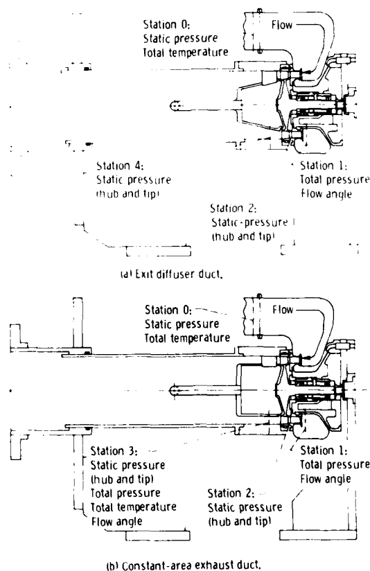
Figure 7. - Turbine instrumentation.
