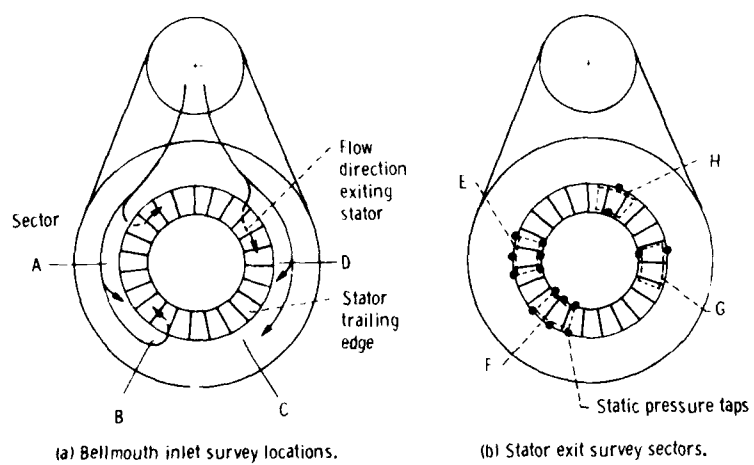
Figure 11. - Bellmouth inlet and stator exit survey locations (view looking into manifold).
