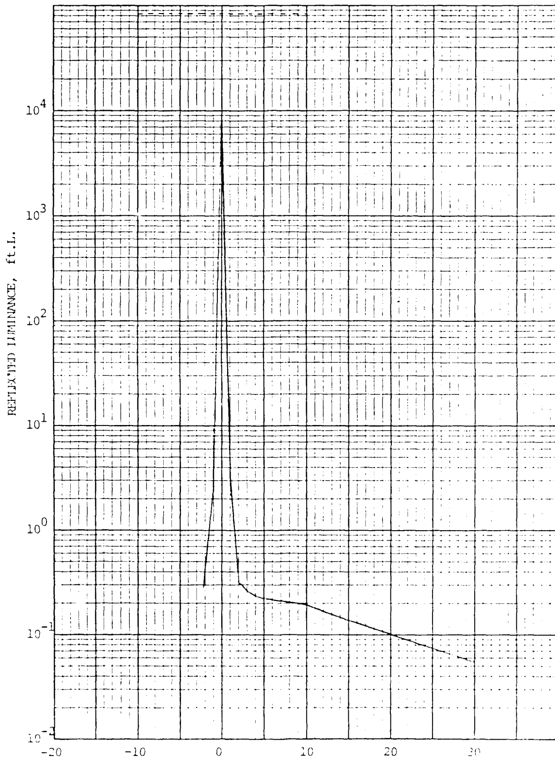
ANGULAR DISPLACEMENT (α), DEGREES Fig. 55 Reflectance, Faceplate No. 90
