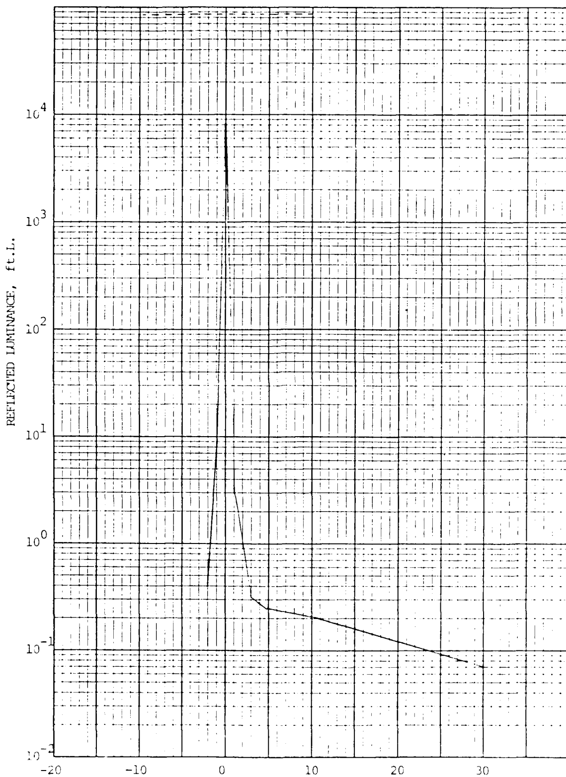
Fig.54 Reflectance, Faceplate No. 89
