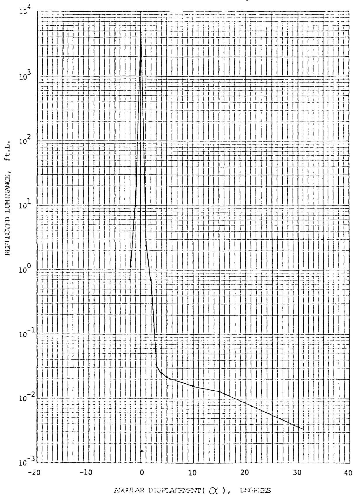
Fig. 30 Reflectance, Faceplate No. 40
