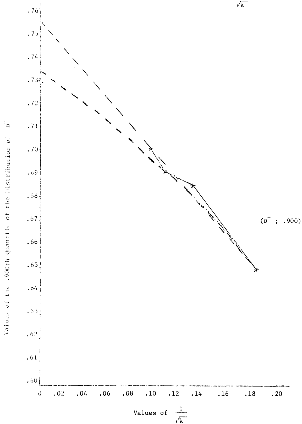
Figure 4.7 Plot of the .900th Quantile of D^- vs \frac{1}{\sqrt{k}}
